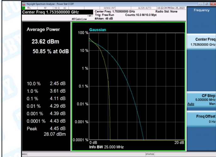
Band4-3MHz-QPSK-20385-15RB#0-PASS
