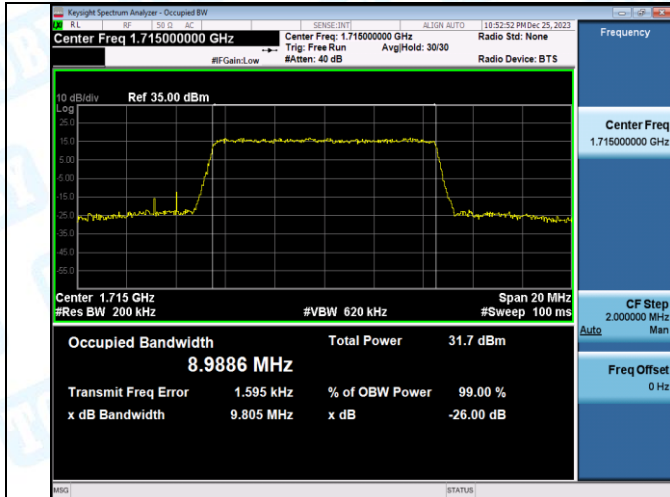
Band4-10MHz-QPSK-20175-50RB#0-PASS
