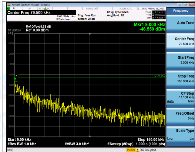
Band4_3MHz_QPSK_19965_1RB#0_30~1000_30~1000
