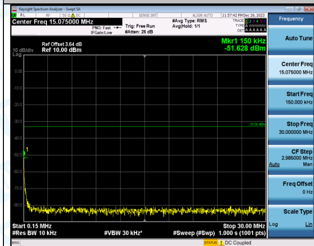
Band4_20MHz_16QAM_20300_1RB#0_1000~3000_1000~3000
