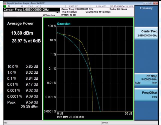
Band41-10MHz-16QAM-41540-50RB#0-PASS
