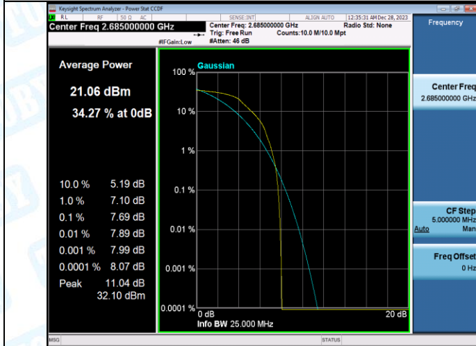
Band41-10MHz-QPSK-41540-50RB#0-PASS
