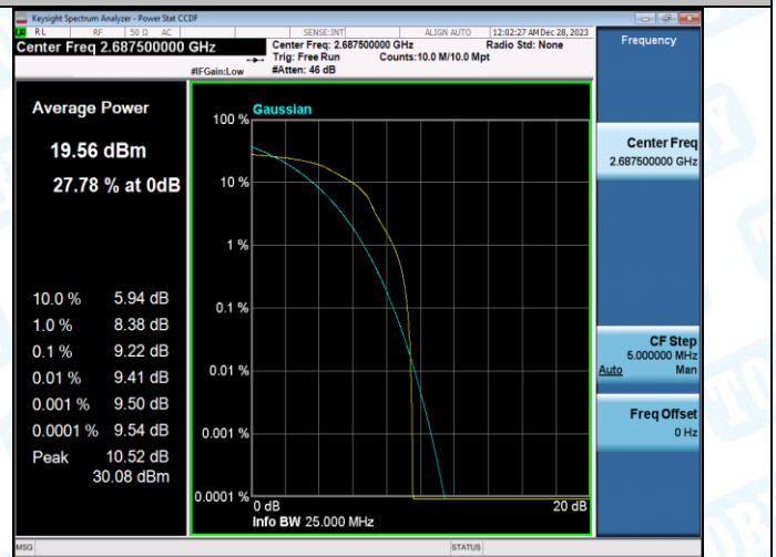
Band41-5MHz-16QAM-41565-25RB#0-PASS
