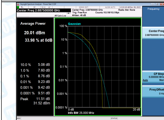
Band41-10MHz-QPSK-39700-1RB#0-PASS
