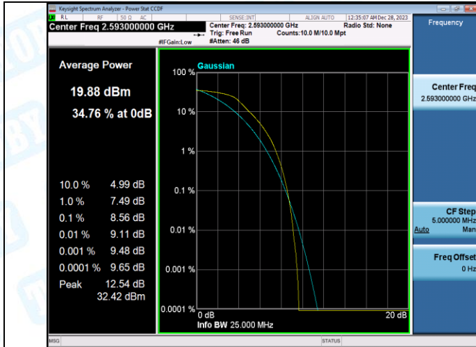
Band41-10MHz-QPSK-41540-1RB#0-PASS
