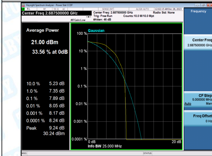
Band41-5MHz-QPSK-41565-25RB#0-PASS
