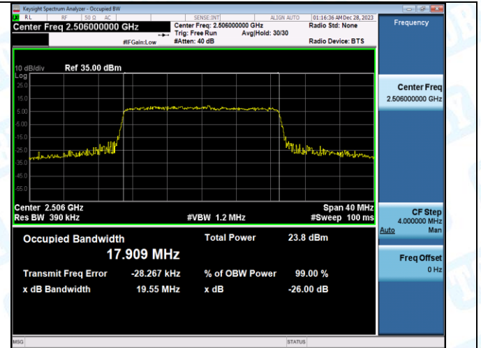
Band41-20MHz-16QAM-40620-100RB#0-PASS
