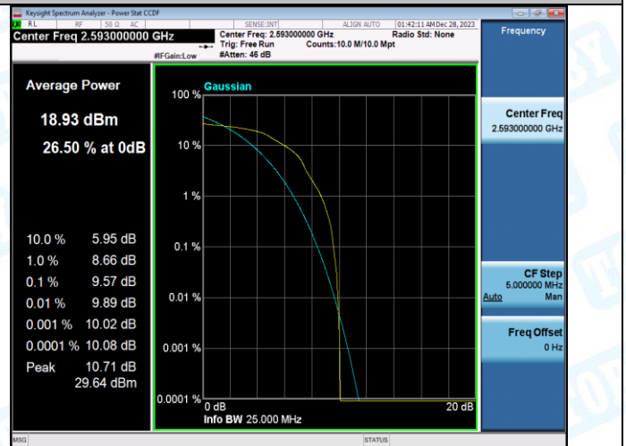
Band41-20MHz-16QAM-40620-100RB#0-PASS
