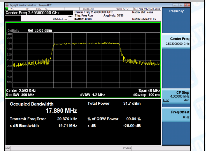
Band41-20MHz-16QAM-41490-100RB#0-PASS
