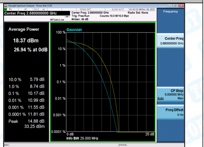
Band41-20MHz-16QAM-41490-100RB#0-PASS
