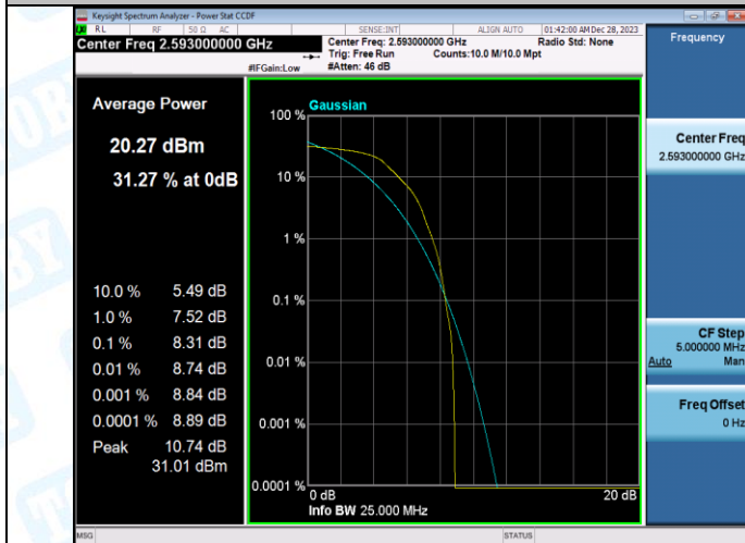
Band41-20MHz-QPSK-40620-100RB#0-PASS
