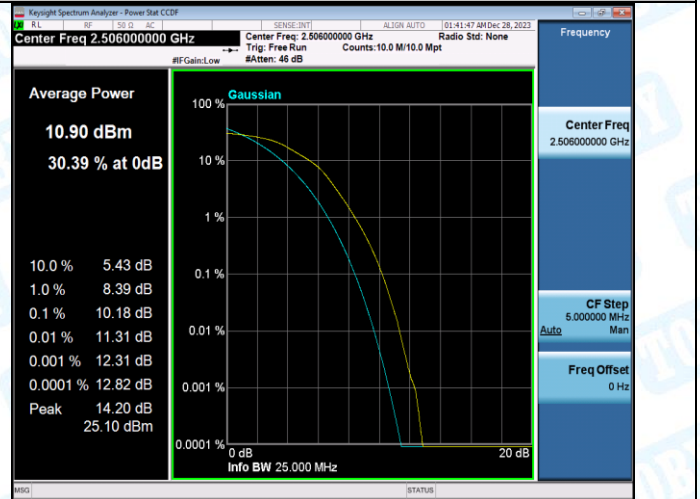
Band41-20MHz-16QAM-40620-1RB#0-PASS
