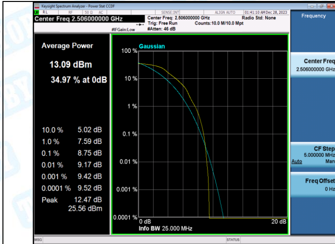
Band41-20MHz-QPSK-39750-100RB#0-PASS
