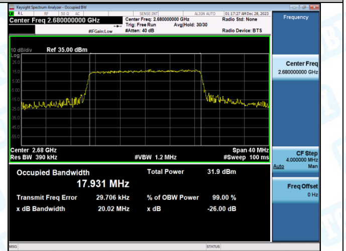
Band41-20MHz-16QAM-41490-100RB#0-PASS
