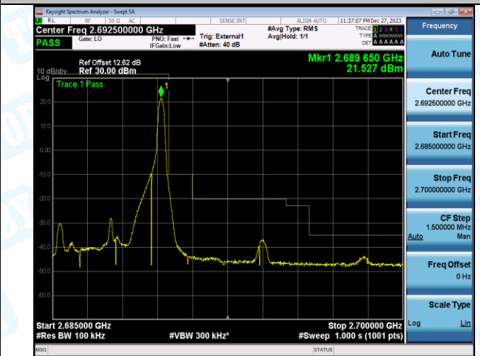
Band41_5MHz_16QAM_41565_25RB#0
