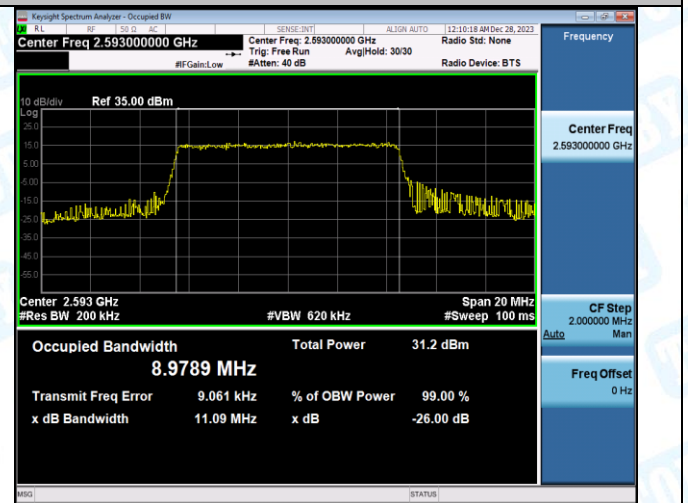
Band41-10MHz-16QAM-41540-50RB#0-PASS
