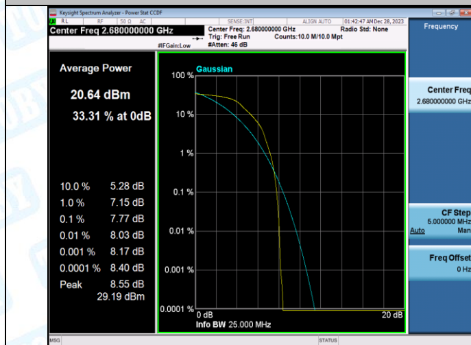
Band41-20MHz-QPSK-41490-100RB#0-PASS
