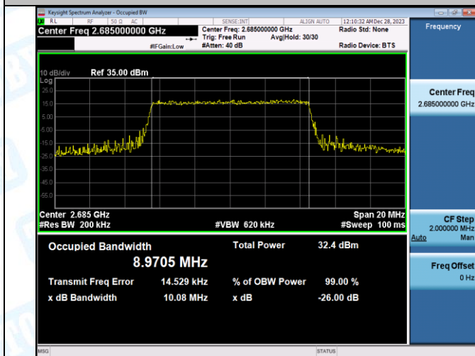
Band41-15MHz-QPSK-39725-75RB#0-PASS
