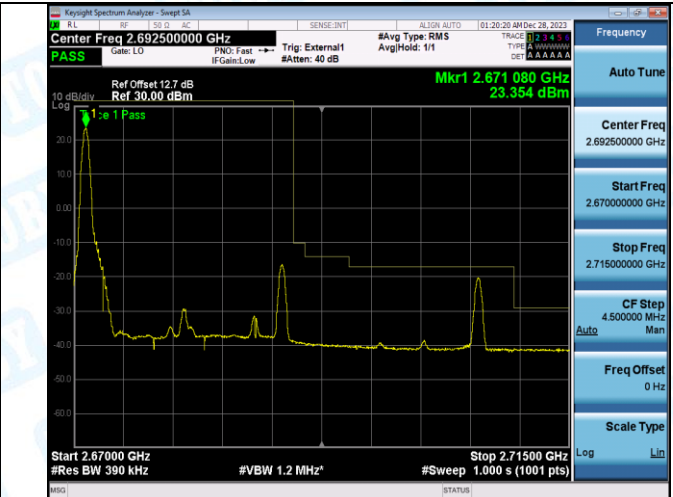
Band41_20MHz_16QAM_41490_1RB#99
