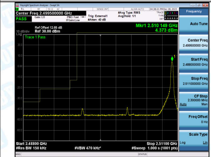
Band41_15MHz_16QAM_39725_75RB#0
