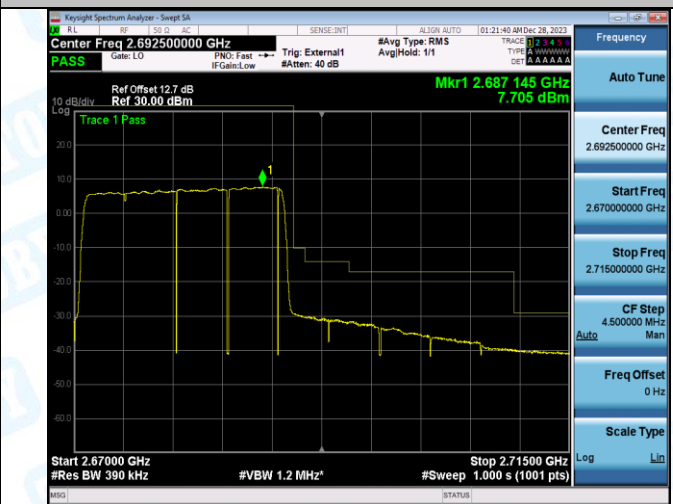
Band41_20MHz_16QAM_41490_100RB#0
