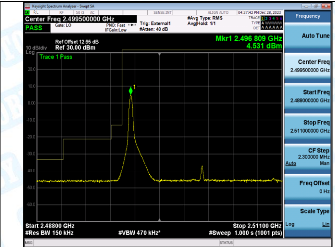
Band41_15MHz_16QAM_39725_1RB#74
