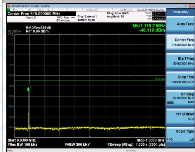
Band41_10MHz_QPSK_41540_1RB#0_20000~27000_20000~27000
