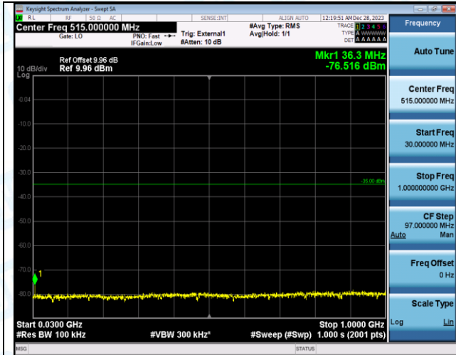
Band41_10MHz_QPSK_40620_1RB#0_20000~27000_20000~27000
