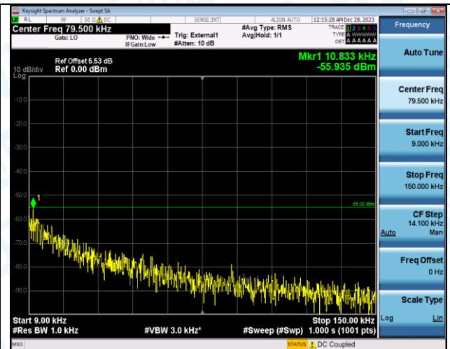
Band41_5MHz_16QAM_41565_1RB#0_0.009~0.15_0.009~0.15
