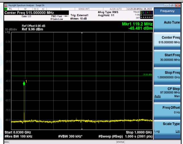
Band41_10MHz_16QAM_41540_1RB#0_20000~27000_20000~27000
