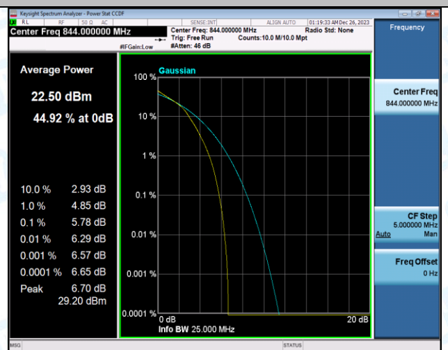
Band5-10MHz-16QAM-20600-50RB#0-PASS
