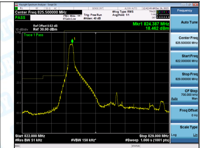
Band5_5MHz_16QAM_20425_1RB#24
