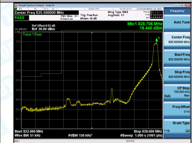
Band5_5MHz_16QAM_20425_25RB#0
