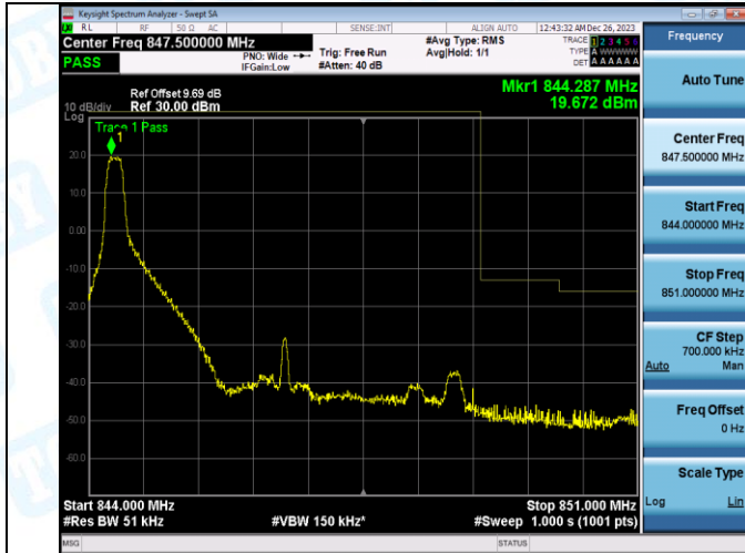
Band5_5MHz_QPSK_20625_1RB#24
