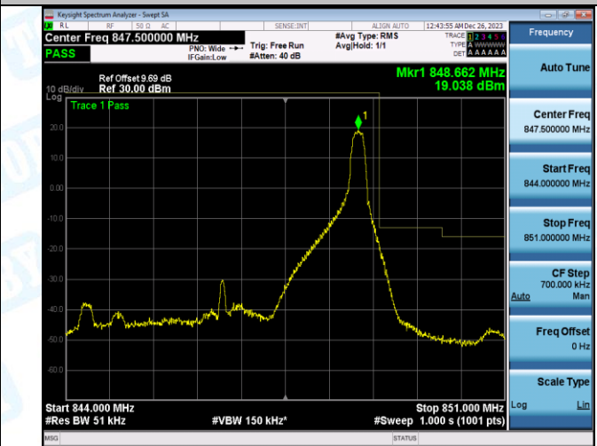
Band5_5MHz_16QAM_20625_25RB#0
