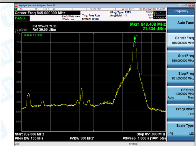
Band5_10MHz_16QAM_20600_50RB#0
