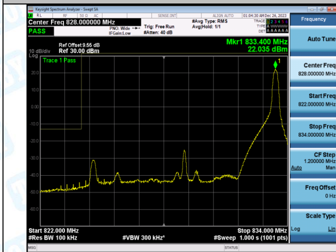
Band5_10MHz_QPSK_20450_50RB#0
