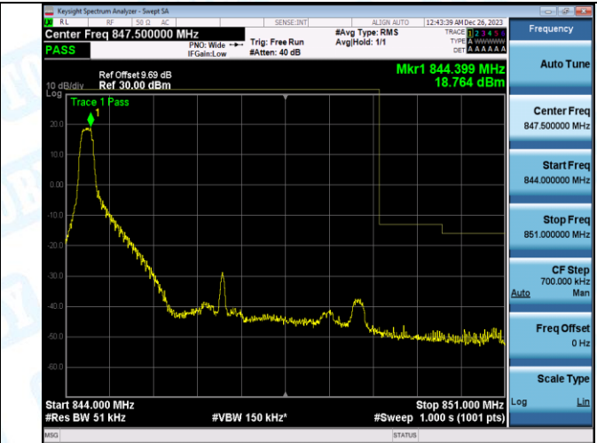
Band5_5MHz_16QAM_20625_1RB#24
