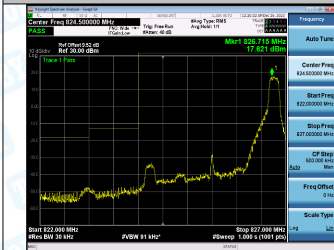
Band5_3MHz_QPSK_20415_15RB#0
