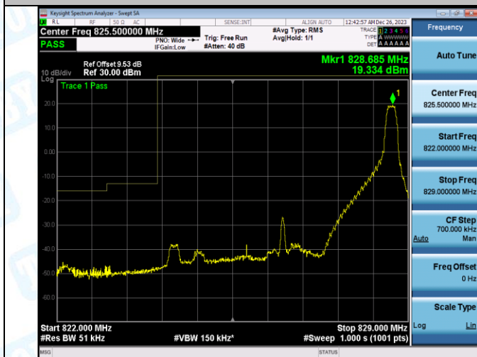
Band5_5MHz_QPSK_20425_25RB#0
