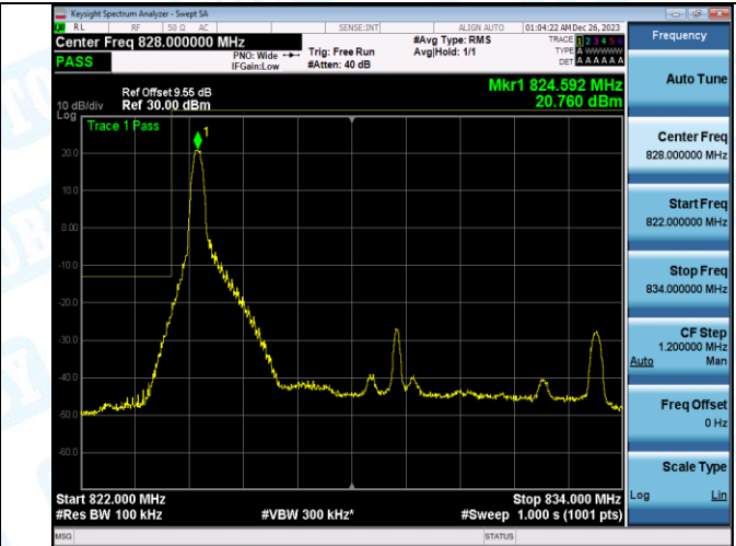
Band5_10MHz_16QAM_20450_1RB#49
