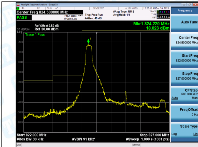
Band5_3MHz_QPSK_20415_1RB#14
