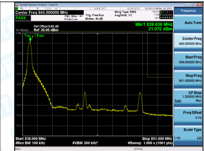
Band5_10MHz_16QAM_20600_1RB#49
