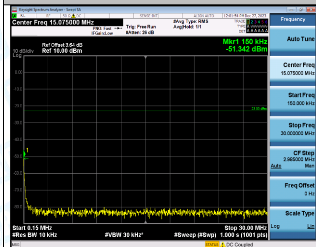
Band5_10MHz_16QAM_20525_1RB#0_1000~3000_1000~3000
