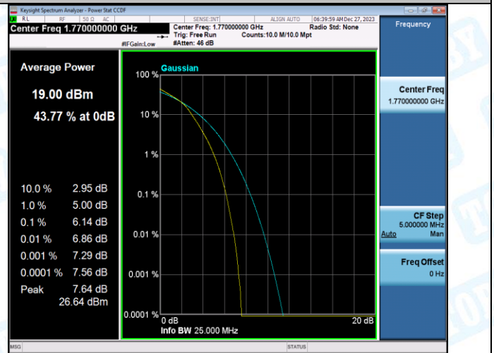
Band66-20MHz-16QAM-132572-100RB#0-PASS
