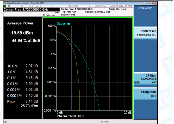
Band66-20MHz-16QAM-132072-100RB#0-PASS
