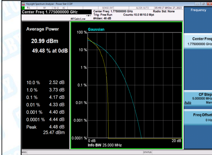
Band66-10MHz-QPSK-132622-50RB#0-PASS
