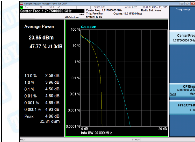
Band66-15MHz-QPSK-132047-75RB#0-PASS
