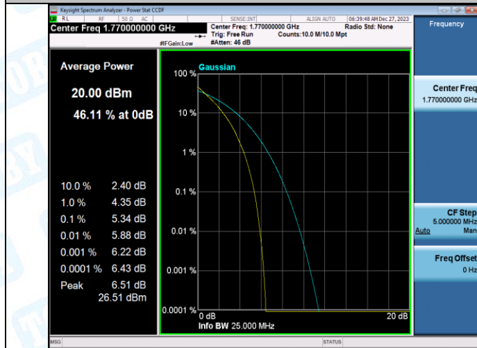
Band66-20MHz-QPSK-132572-100RB#0-PASS
