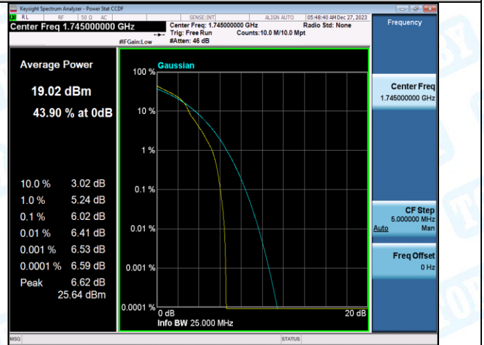
Band66-10MHz-16QAM-132322-50RB#0-PASS
