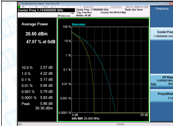
Band66-15MHz-QPSK-132322-75RB#0-PASS
