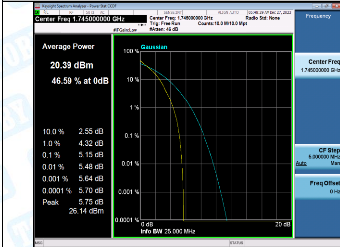
Band66-10MHz-QPSK-132322-50RB#0-PASS
