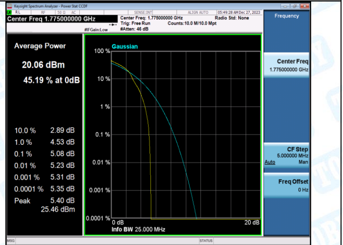
Band66-10MHz-16QAM-132622-50RB#0-PASS
