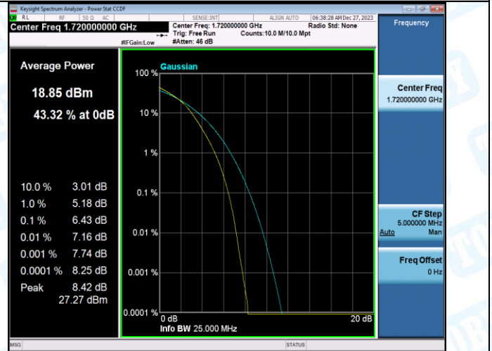
Band66-20MHz-16QAM-132322-1RB#0-PASS
