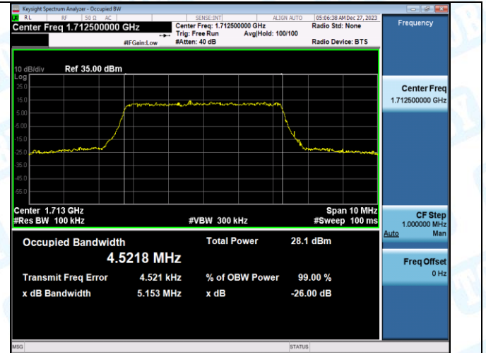
Band66-5MHz-16QAM-132322-25RB#0-PASS
