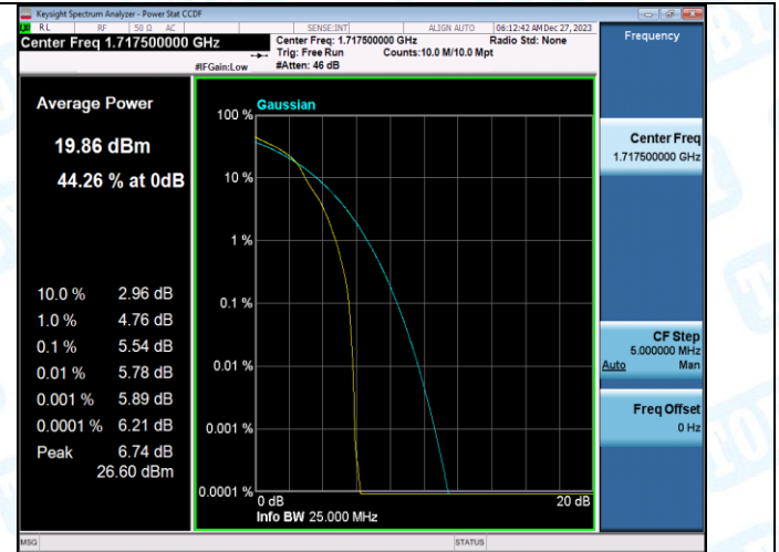
Band66-15MHz-16QAM-132047-75RB#0-PASS
