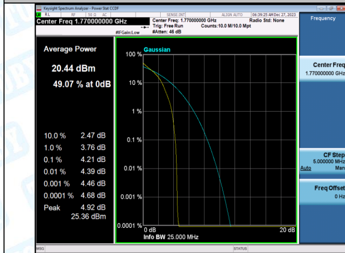
Band66-20MHz-QPSK-132572-100RB#0-PASS
