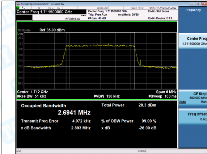
Band66-3MHz-QPSK-132322-15RB#0-PASS
