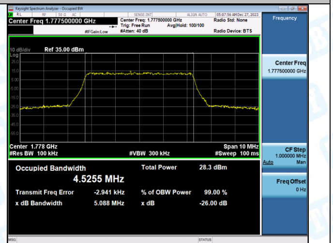
Band66-10MHz-16QAM-132022-50RB#0-PASS
