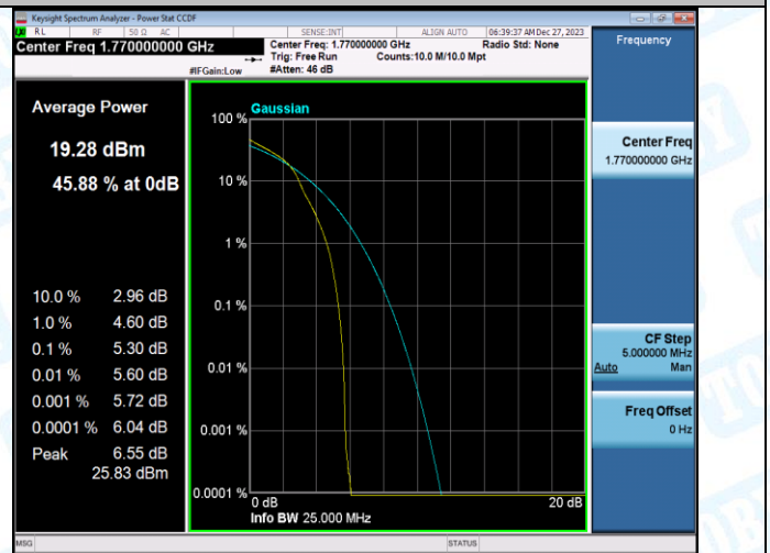
Band66-20MHz-16QAM-132572-100RB#0-PASS
