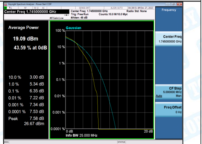
Band66-20MHz-16QAM-132322-100RB#0-PASS
