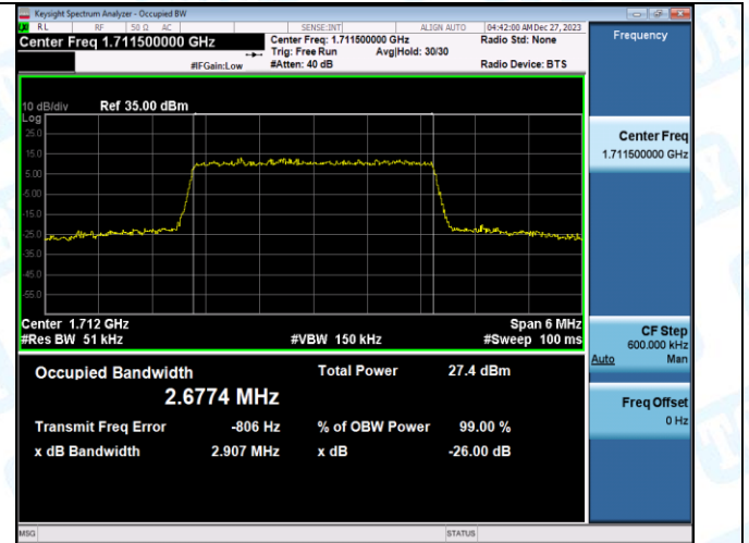
Band66-3MHz-16QAM-132322-15RB#0-PASS
