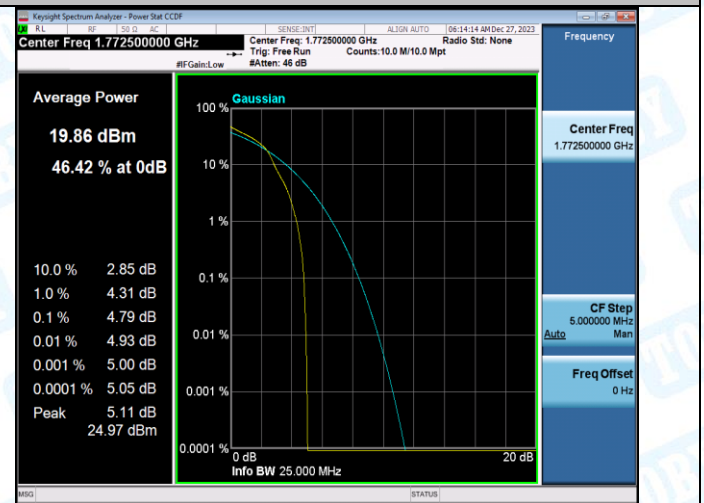
Band66-15MHz-16QAM-132597-75RB#0-PASS
