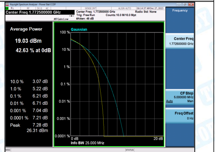
Band66-20MHz-16QAM-132072-1RB#0-PASS
