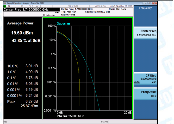
Band66-10MHz-16QAM-132022-50RB#0-PASS
