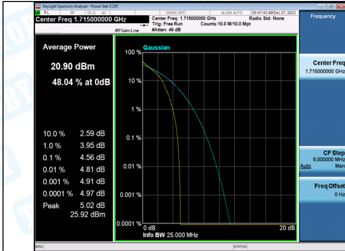
Band66-10MHz-QPSK-132022-50RB#0-PASS
