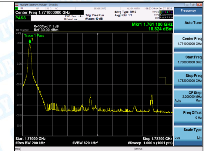
Band66_20MHz_16QAM_132572_1RB#99
