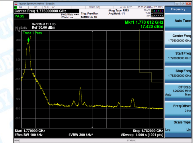
Band66_10MHz_16QAM_132622_1RB#49
