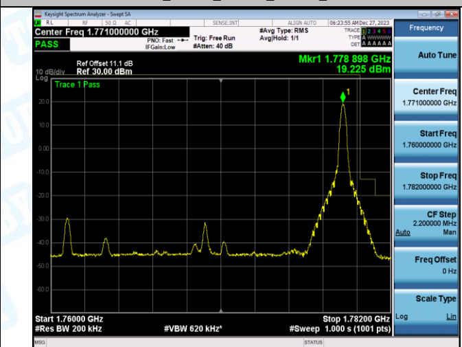
Band66_20MHz_16QAM_132572_100RB#0
