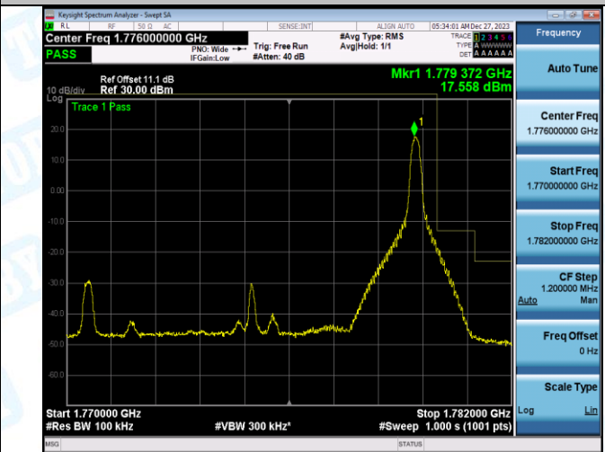
Band66_10MHz_16QAM_132622_50RB#0
