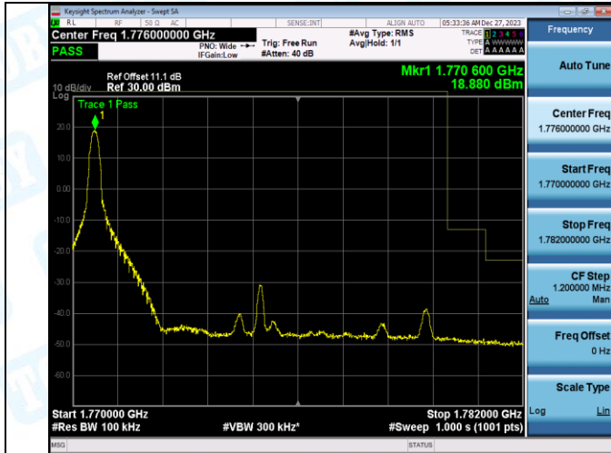
Band66_10MHz_QPSK_132622_1RB#49
