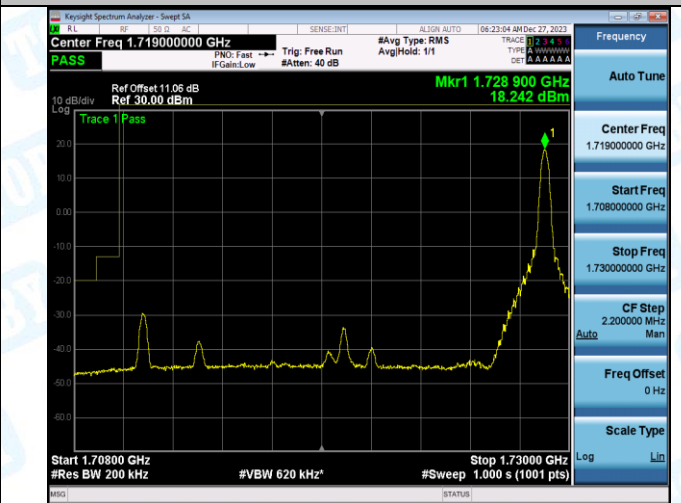
Band66_20MHz_16QAM_132072_100RB#0
