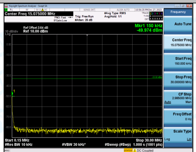
Band66_3MHz_QPSK_132322_1RB#0_1000~3000_1000~3000
