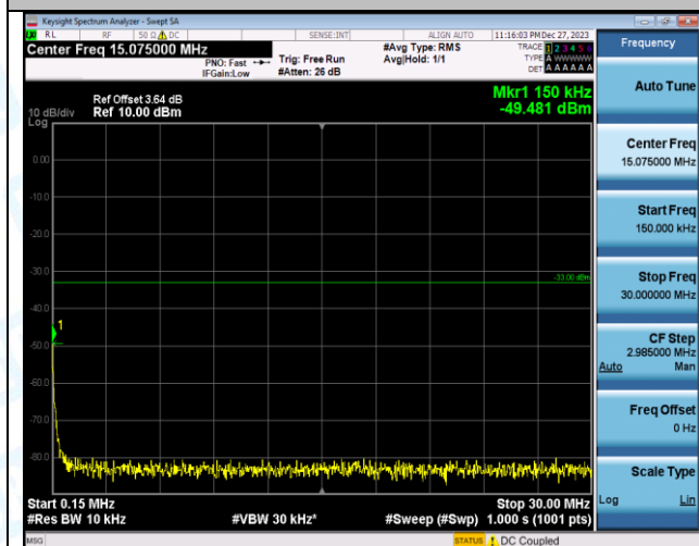
Band66_15MHz_16QAM_132322_1RB#0_1000~3000_1000~3000
