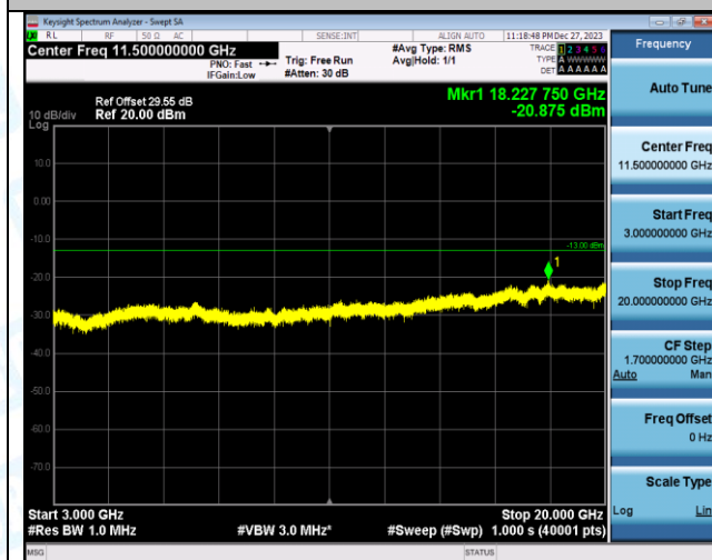
Band66_20MHz_QPSK_132072_1RB#0_0.15~30_0.15~30
