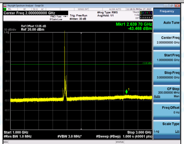
Band66_15MHz_16QAM_132597_1RB#0_1000~3000_1000~3000
