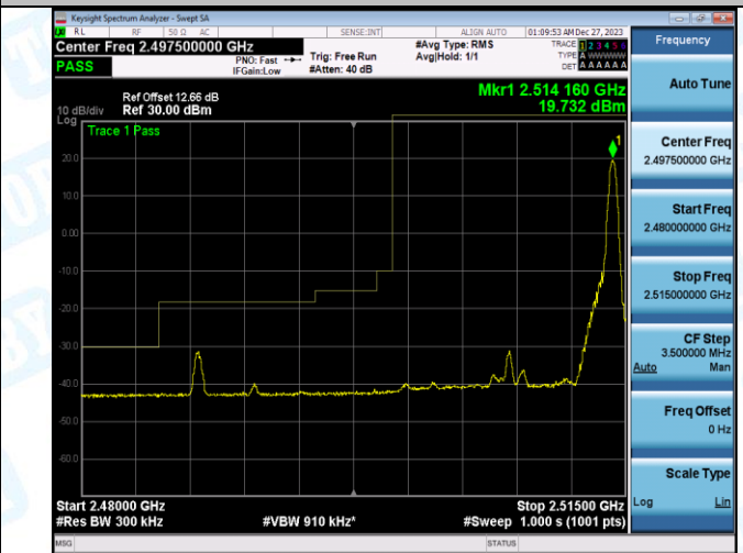
Band7_15MHz_16QAM_20825_75RB#0
