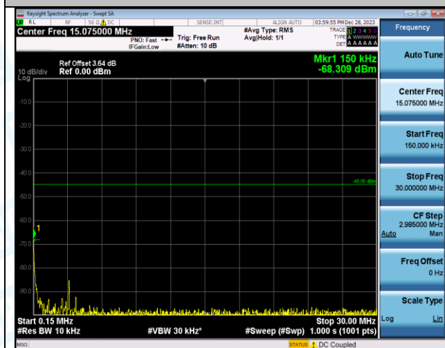
Band7_5MHz_16QAM_21100_1RB#0_0.15~30_0.15~30
