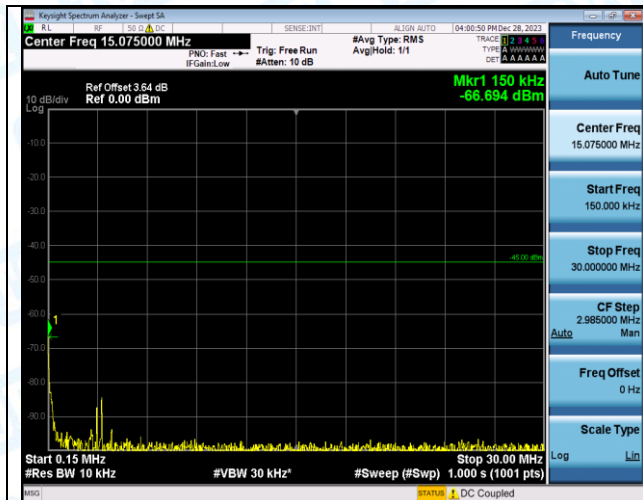
Band7_5MHz_QPSK_21100_1RB#0_20000~27000_20000~27000
