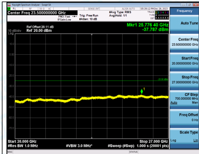
Band7_5MHz_16QAM_20775_1RB#0_20000~27000_20000~27000
