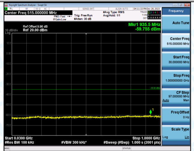
Band7_15MHz_QPSK_21100_1RB#0_30~1000_30~1000
