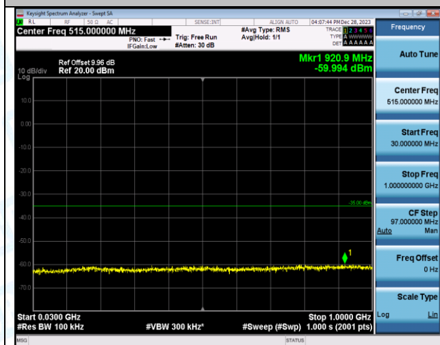
Band7_10MHz_16QAM_21400_1RB#0_30~1000_30~1000
