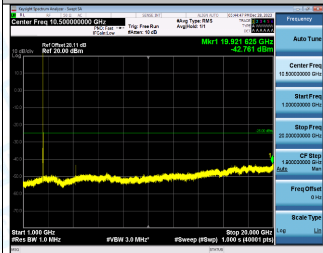
Band7_15MHz_16QAM_20825_1RB#0_1000~20000_1000~20000
