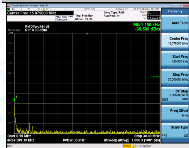
Band7_15MHz_16QAM_21375_1RB#0_0.15~30_0.15~30
