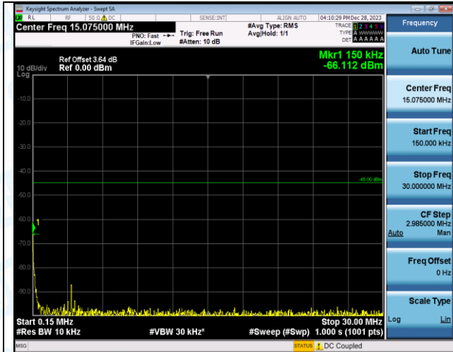
Band7_15MHz_QPSK_21100_1RB#0_0.15~30_0.15~30
