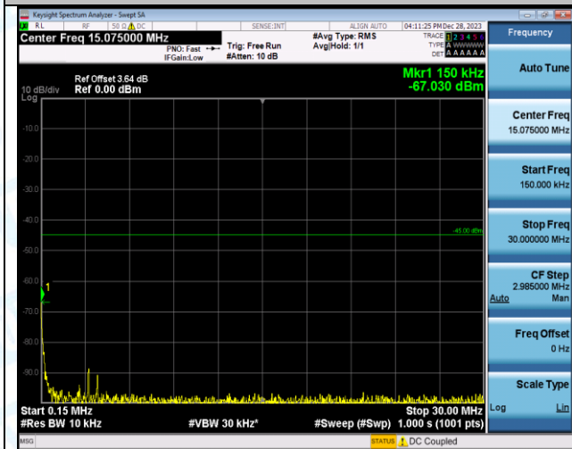
Band7_15MHz_QPSK_21100_1RB#0_0.15~30_0.15~30
