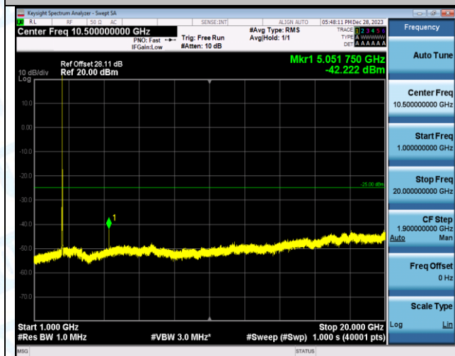
Band7_20MHz_QPSK_21350_1RB#0_1000~20000_1000~20000
