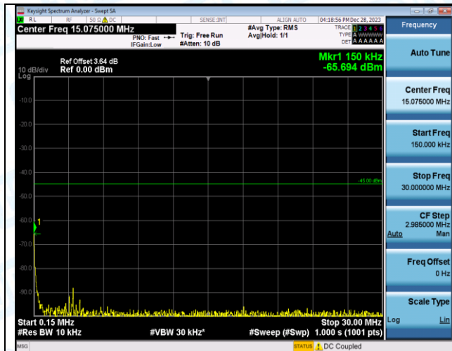
Band7_20MHz_16QAM_21100_1RB#0_1000~20000_1000~20000
