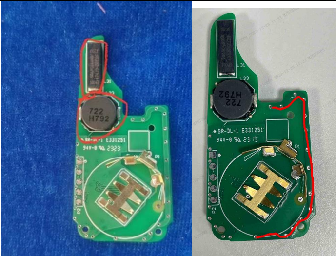
LF antenna
