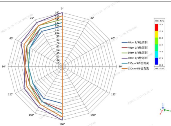
LF antenna
