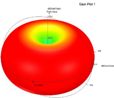
RF antenna
