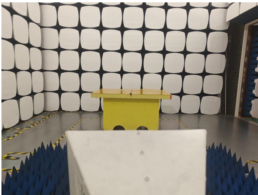
RE 1GHz-6GHz
