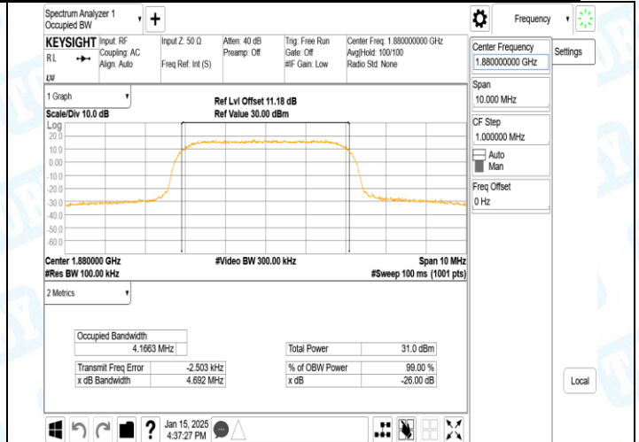
Band2-9400-3-PASS
