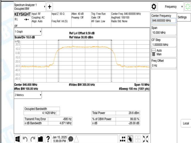
Band5-4233-3-PASS
