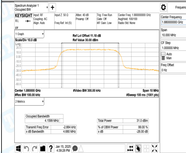
Band2-9400-2-PASS
