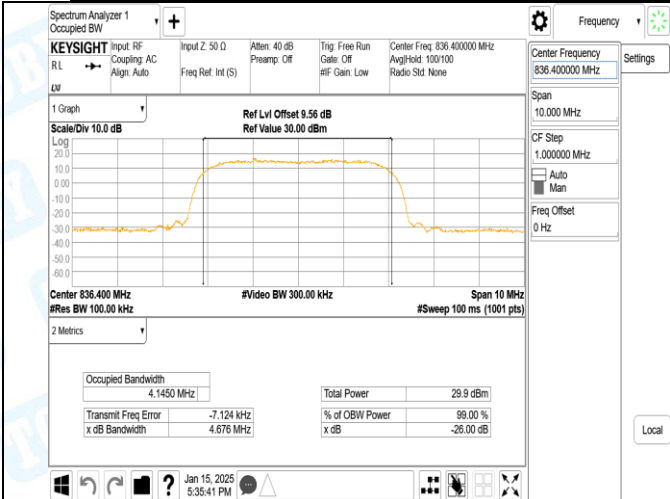
Band5-4182-3-PASS
