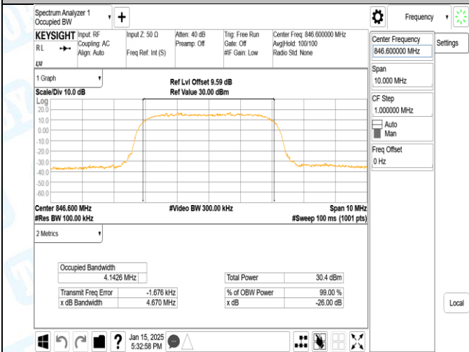
Band5-4233-1-PASS
