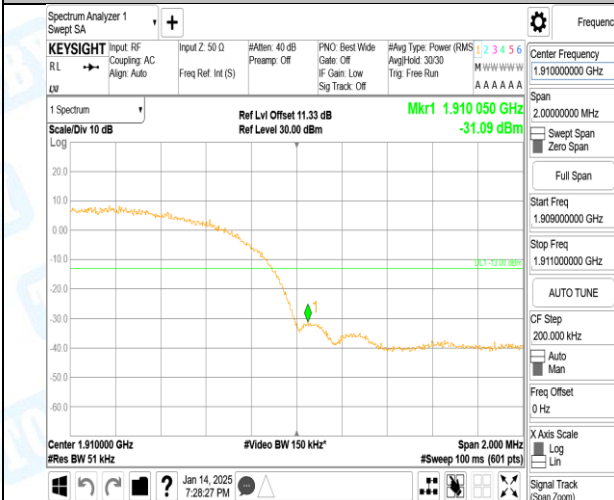
Band2-9538-1-PASS
