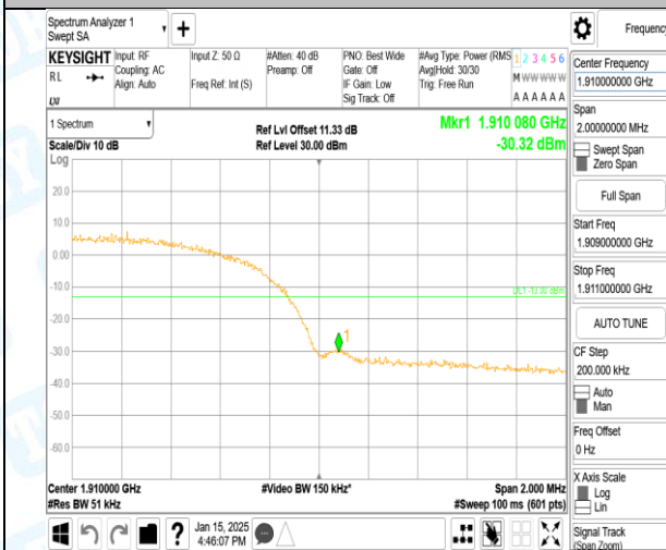
Band2-9538-4-PASS
