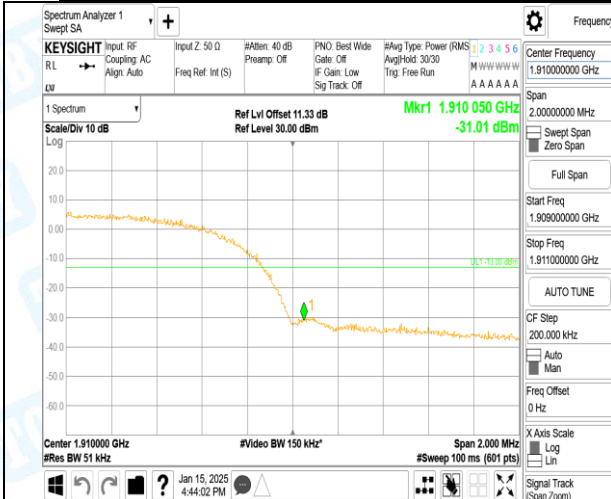
Band2-9538-2-PASS
