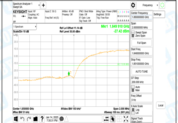
Band2-9262-4-PASS
