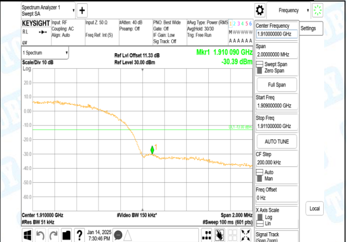
Band2-9538-4-PASS
