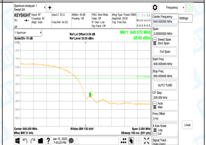
Band5-4233-1-PASS
