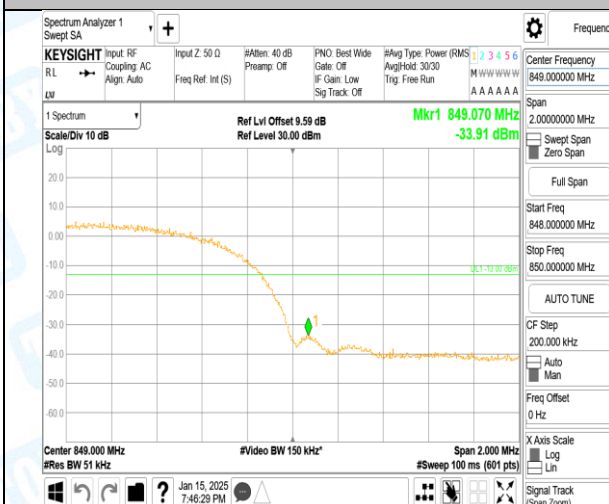
Band5-4233-2-PASS
