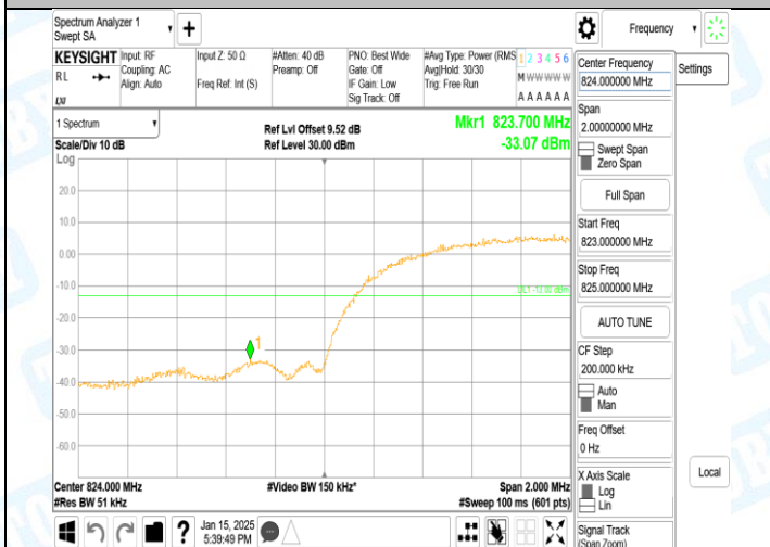
Band5-4132-3-PASS
