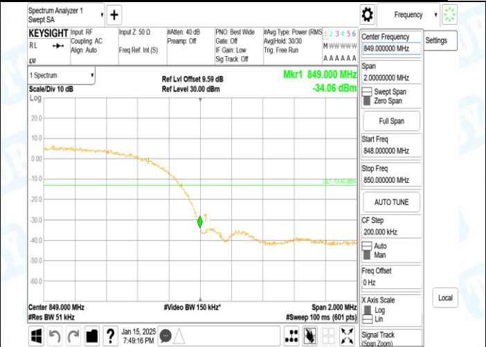
Band5-4233-5-PASS
