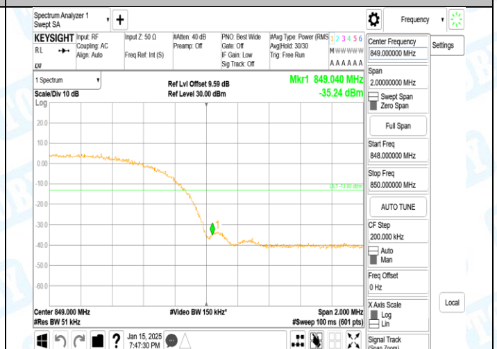
Band5-4233-3-PASS
