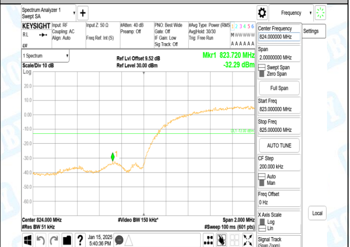
Band5-4132-4-PASS
