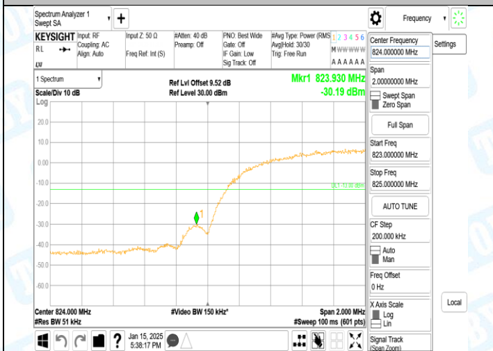
Band5-4132-1-PASS
