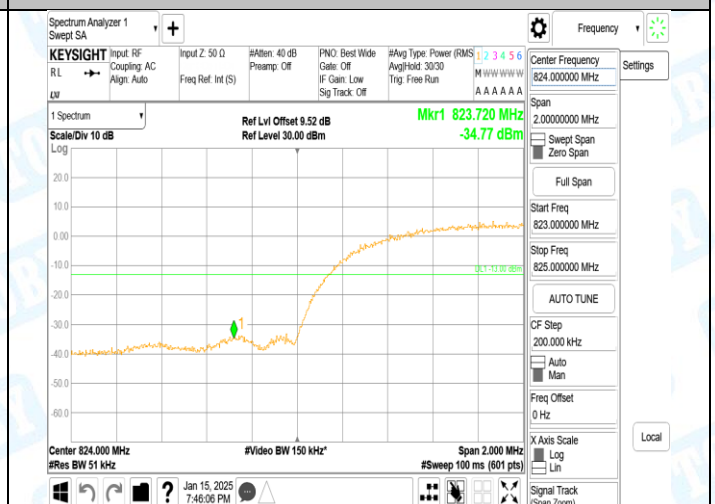
Band5-4132-2-PASS
