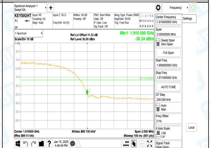
Band2-9538-5-PASS
