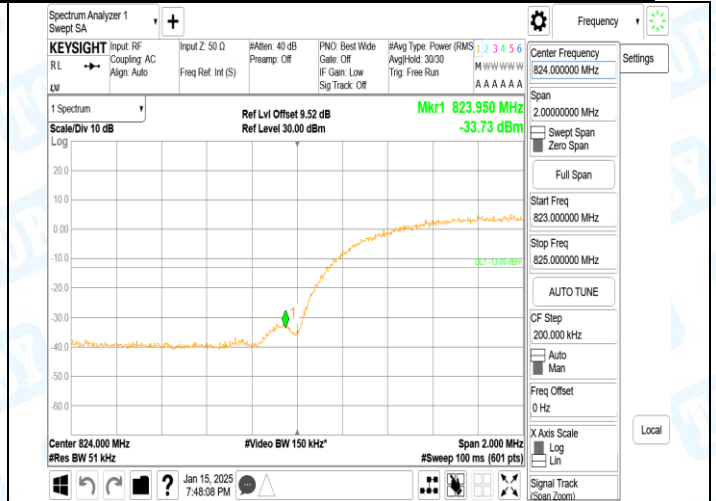
Band5-4132-4-PASS
