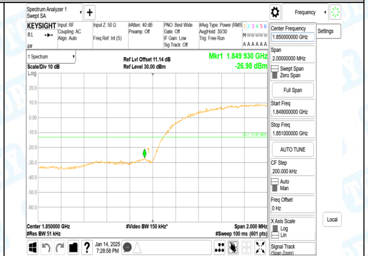
Band2-9262-2-PASS
