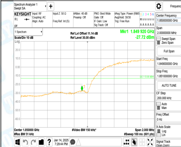
Band2-9262-3-PASS
