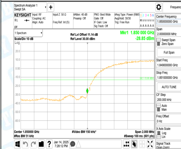
Band2-9262-1-PASS
