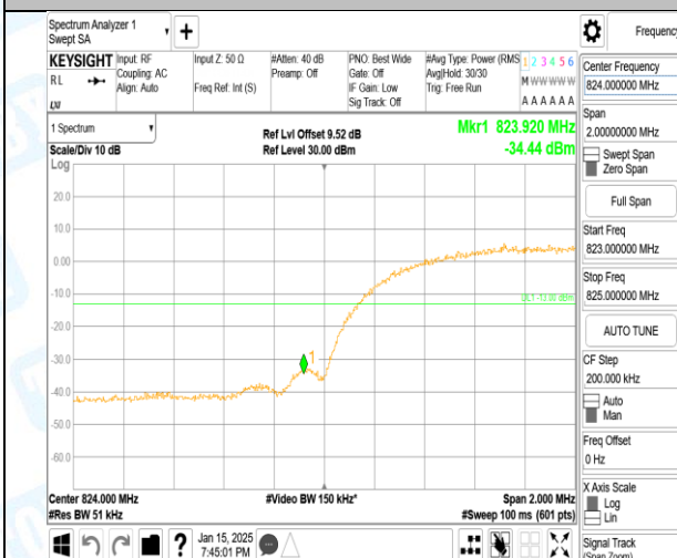
Band5-4132-1-PASS
