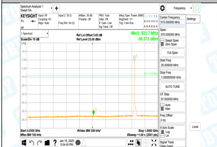
Band5-4132-30~1000MHz-PASS
