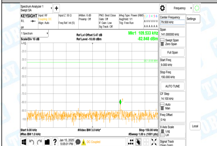
Band5-4182-0.009~0.15MHz-PASS
