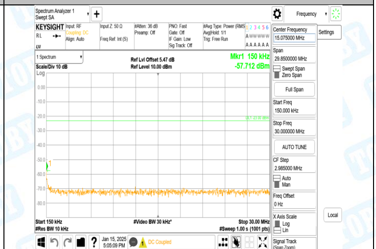
Band5-4182-0.15~30MHz-PASS
