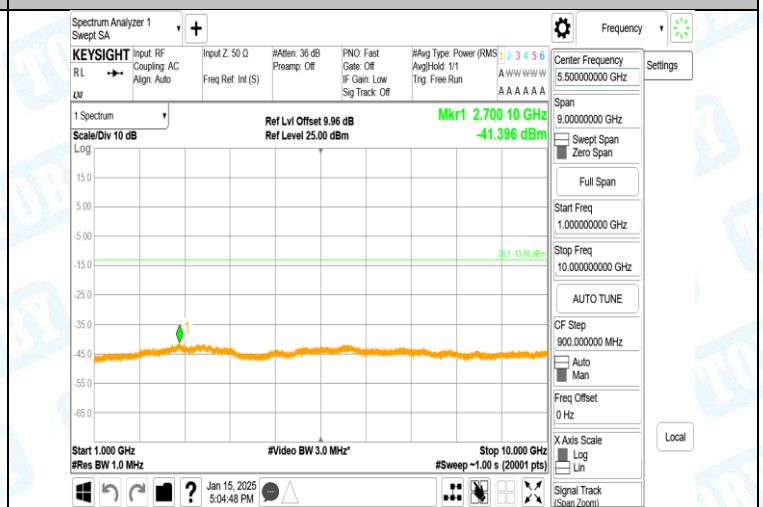
Band5-4132-1000~10000MHz-PASS
