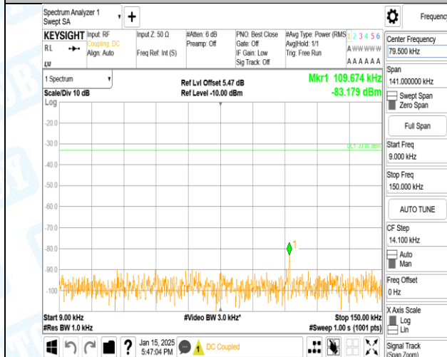
Band5-4233-3-0.009~0.15MHz-PASS
