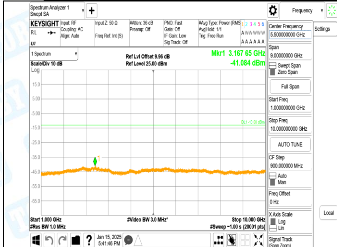
Band5-4132-1-1000~10000MHz-PASS
