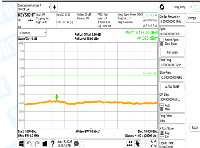
Band5-4132-3-1000~10000MHz-PASS
