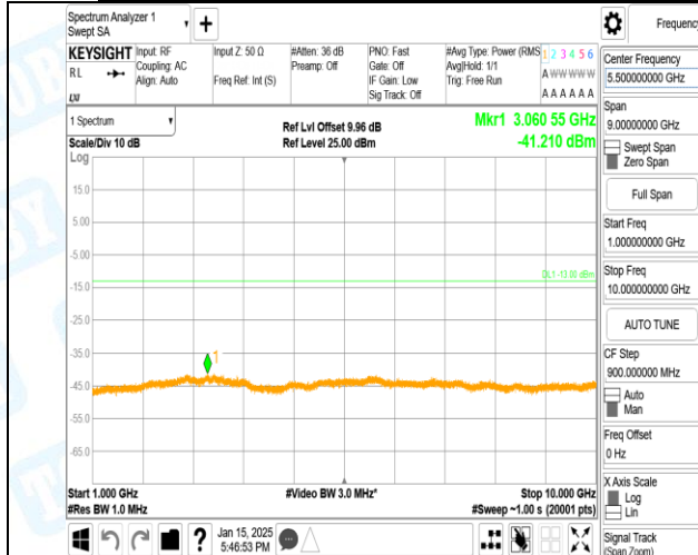
Band5-4182-3-1000~10000MHz-PASS
