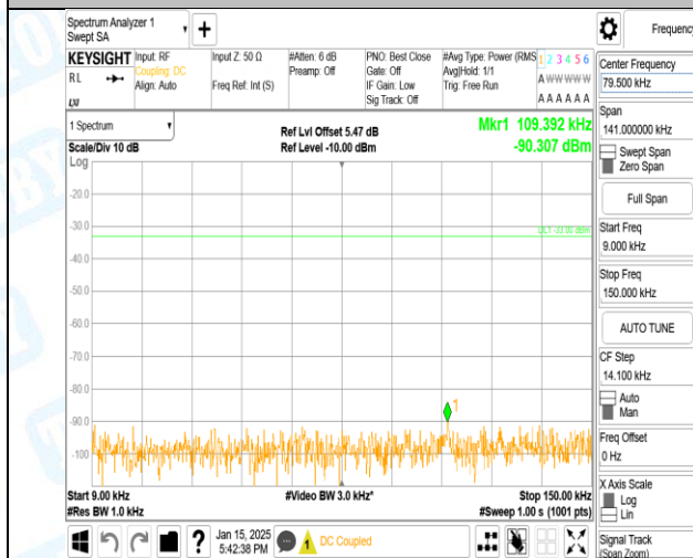
Band5-4233-1-0.009~0.15MHz-PASS
