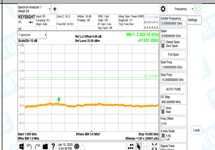
Band5-4182-2-1000~10000MHz-PASS
