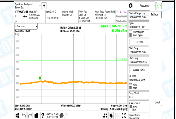
Band5-4132-4-1000~10000MHz-PASS
