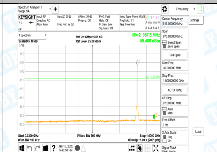
Band5-4182-4-30~1000MHz-PASS
