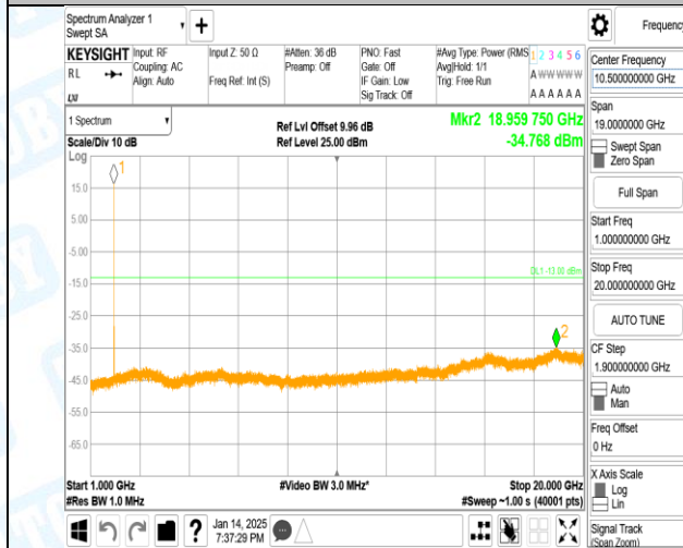
Band2-9538-3-1000~20000MHz-PASS
