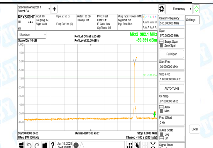
Band5-4182-2-30~1000MHz-PASS
