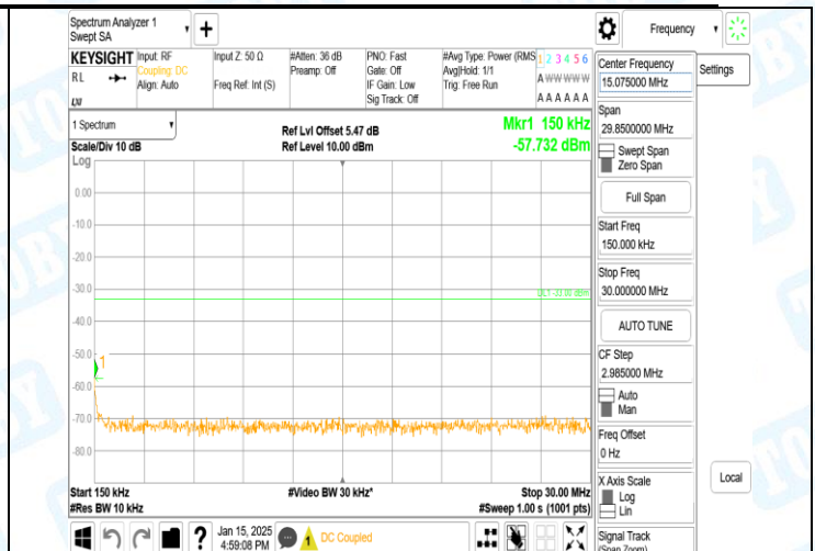
Band2-9538-5-0.15~30MHz-PASS
