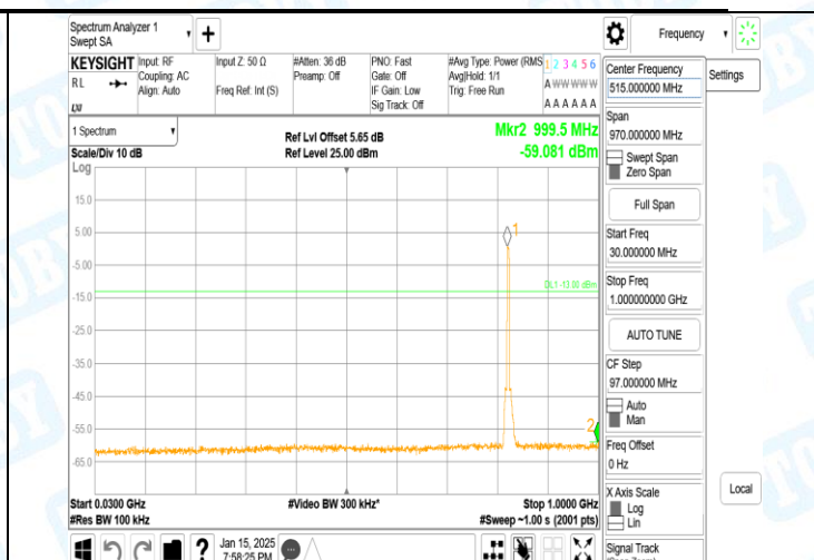
Band5-4132-4-30~1000MHz-PASS
