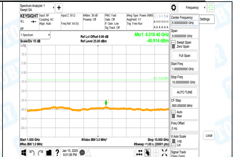
Band5-4132-5-1000~10000MHz-PASS
