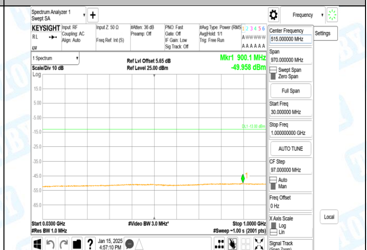
Band2-9538-4-30~1000MHz-PASS
