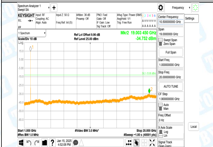
Band2-9538-2-1000~20000MHz-PASS
