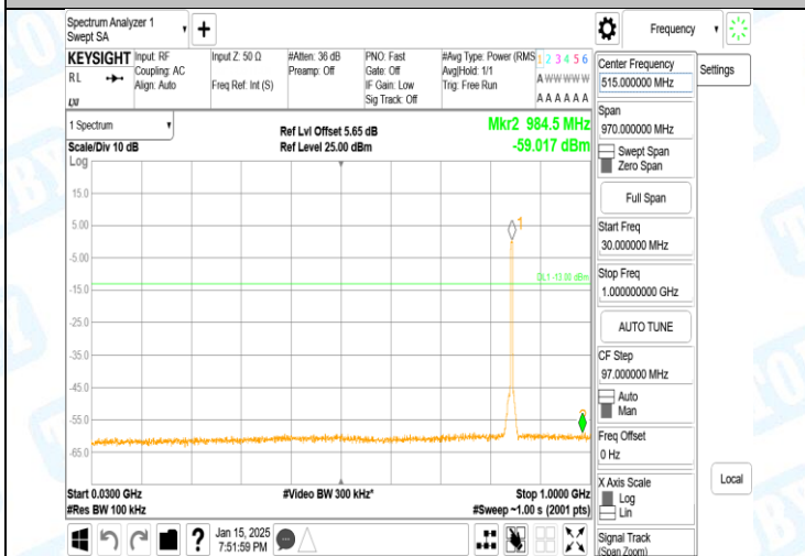
Band5-4233-1-30~1000MHz-PASS
