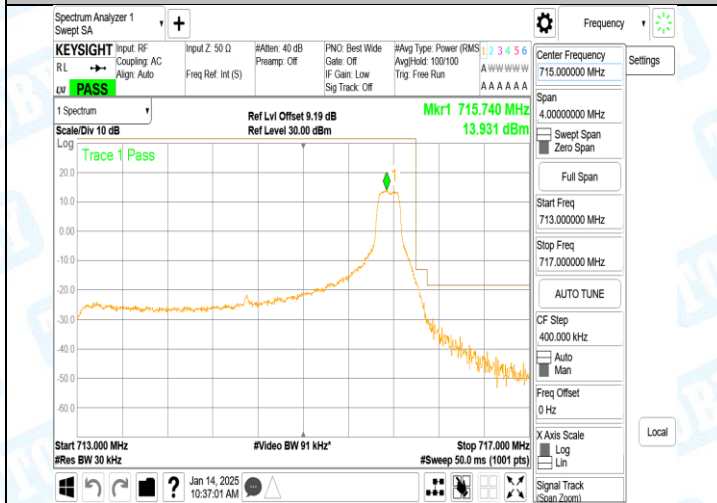
Band12_3MHz_16QAM_23165_1RB#14
