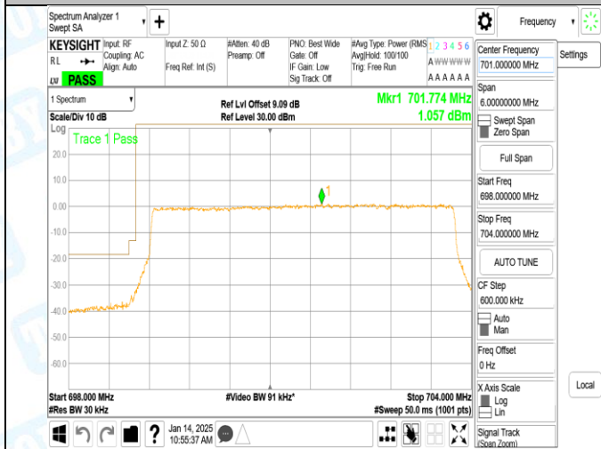
Band12_5MHz_QPSK_23035_25RB#0
