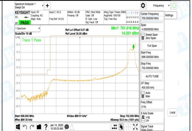
Band12_3MHz_16QAM_23025_1RB#14
