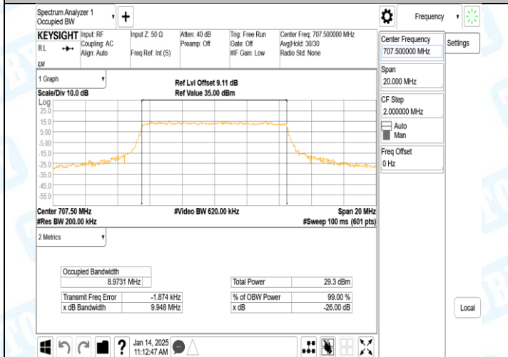
Band12-10MHz-16QAM-23095-50RB#0-PASS
