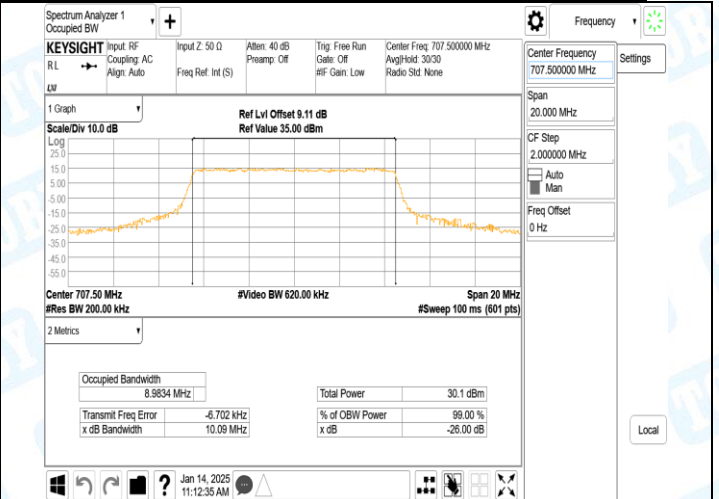
Band12-10MHz-QPSK-23095-50RB#0-PASS
