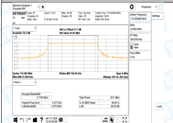
Band12-3MHz-QPSK-23165-15RB#0-PASS
