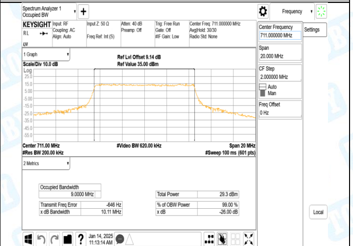
Band12-10MHz-16QAM-23130-50RB#0-PASS
