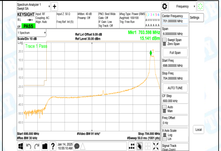
Band12_5MHz_QPSK_23035_1RB#24
