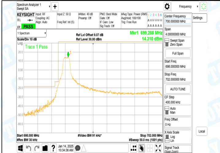
Band12_3MHz_16QAM_23025_1RB#0
