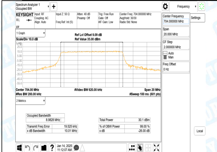
Band12-10MHz-QPSK-23060-50RB#0-PASS
