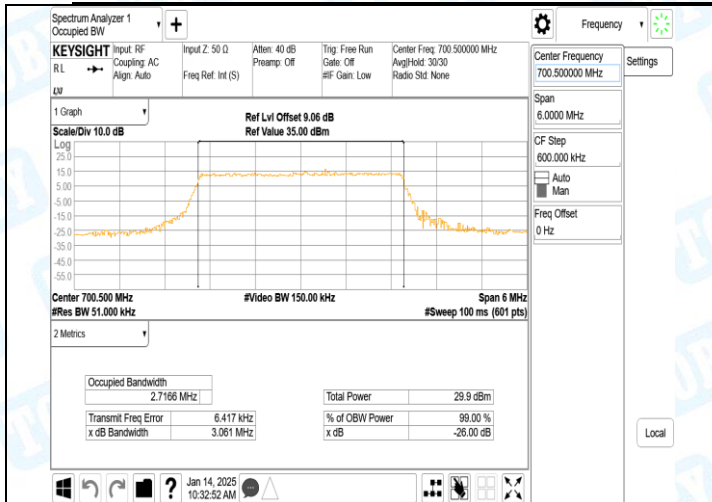
Band12-3MHz-QPSK-23025-15RB#0-PASS
