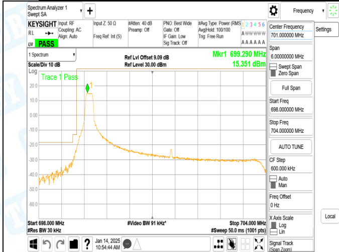
Band12_5MHz_QPSK_23035_1RB#0
