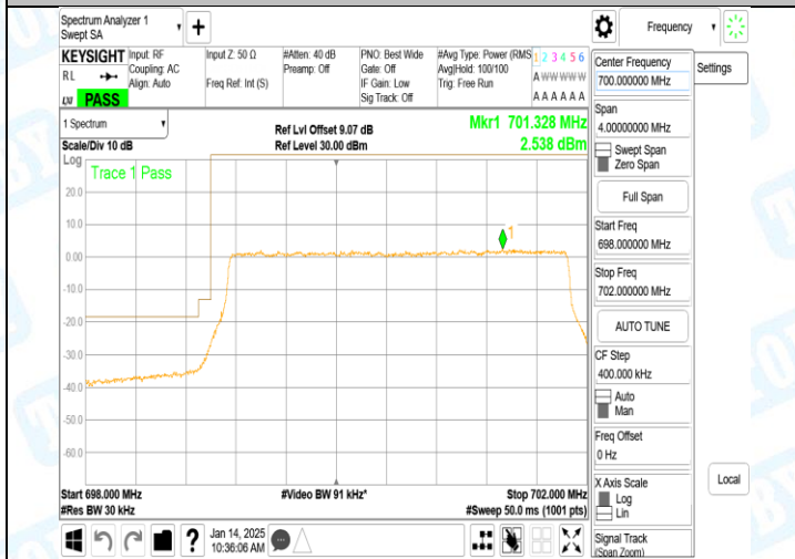
Band12_3MHz_16QAM_23025_15RB#0
