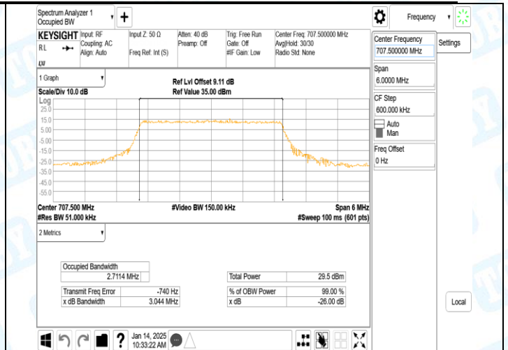
Band12-3MHz-QPSK-23095-15RB#0-PASS
