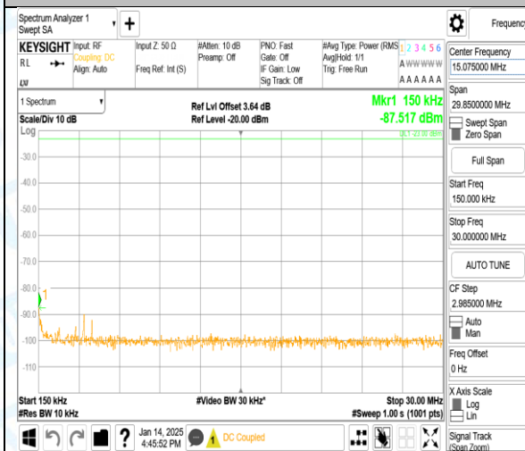
Band17_10MHz_16QAM_23800_1RB#0_0.15~30_0.15~30
