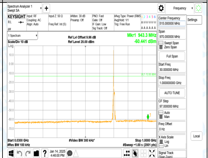
Band17_10MHz_16QAM_23800_1RB#0_30~1000_30~1000
