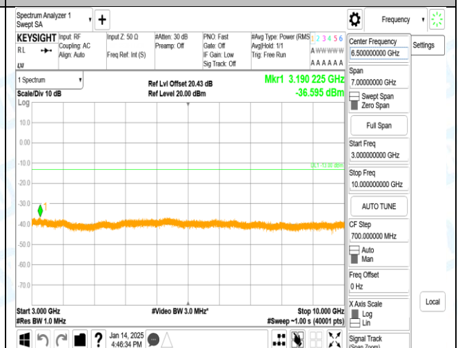
Band17_10MHz_16QAM_23800_1RB#0_3000~10000_3000~10000
