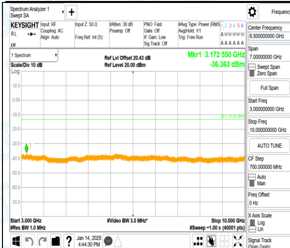
Band17_10MHz_16QAM_23790_1RB#0_3000~10000_3000~10000
