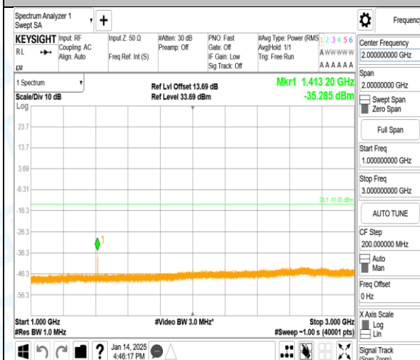
Band17_10MHz_16QAM_23800_1RB#0_1000~3000_1000~3000
