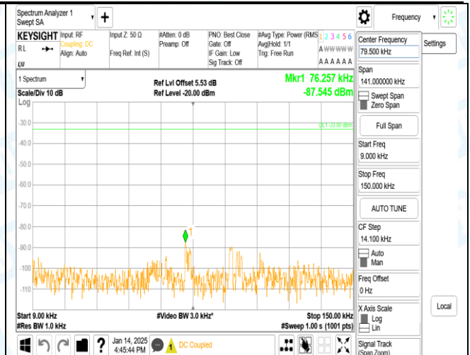
Band17_10MHz_16QAM_23800_1RB#0_0.009~0.15_0.009~0.15
