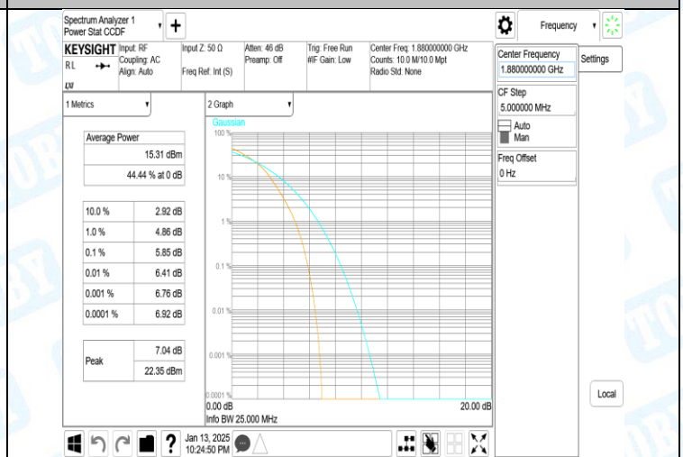
Band2-20MHz-16QAM-18900-100RB#0-PASS
