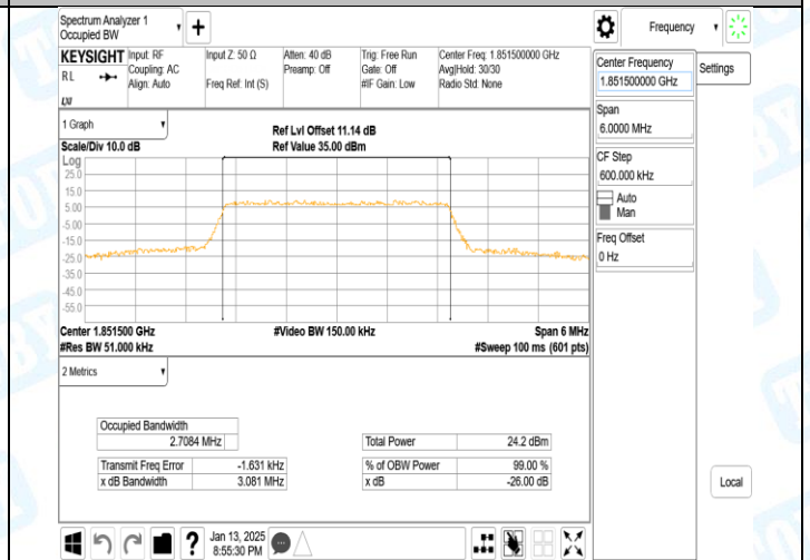
Band2-3MHz-16QAM-18615-15RB#0-PASS
