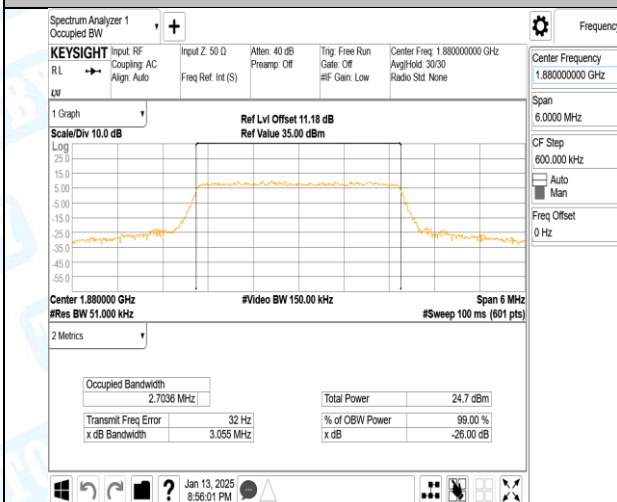
Band2-3MHz-16QAM-18900-15RB#0-PASS
