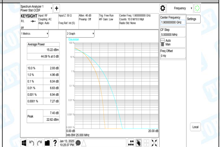
Band2-20MHz-16QAM-19100-100RB#0-PASS
