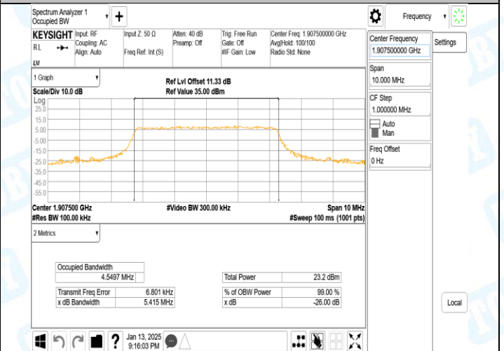
Band2-5MHz-16QAM-19175-25RB#0-PASS
