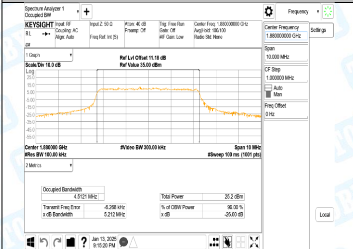
Band2-5MHz-16QAM-18900-25RB#0-PASS
