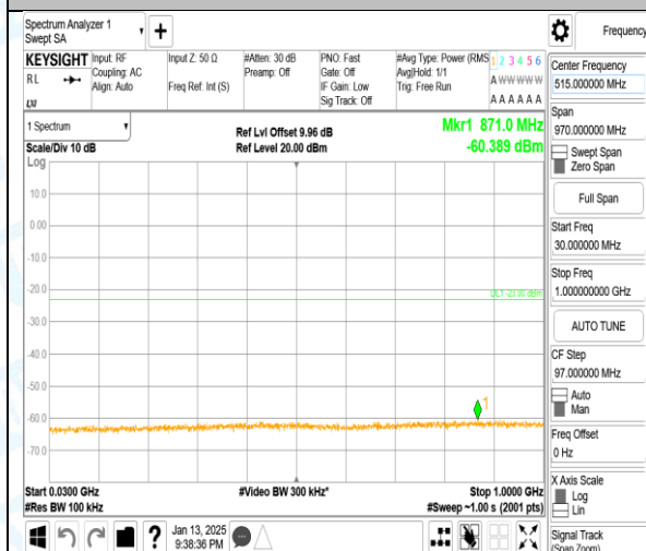
Band2_10MHz_QPSK_18650_1RB#0_30-1000_30-1000
