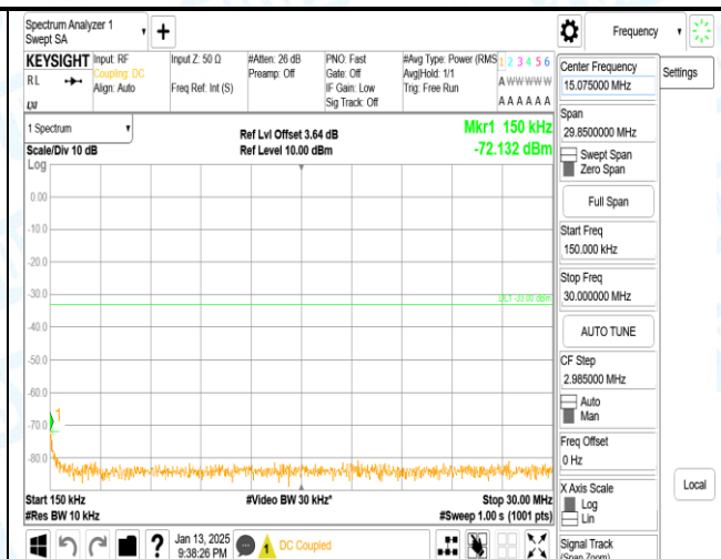
Band2_10MHz_QPSK_18650_1RB#0_0.15-30_0.15-30
