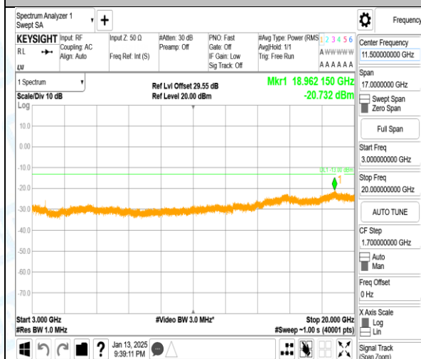
Band2_10MHz_QPSK_18650_1RB#0_3000-20000_3000-20000
