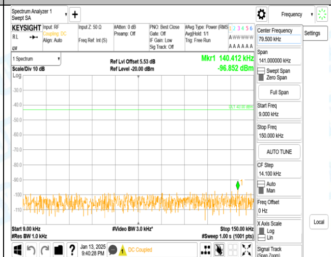
Band2_10MHz_QPSK_18900_1RB#0_0.009-0.15_0.009-0.15
