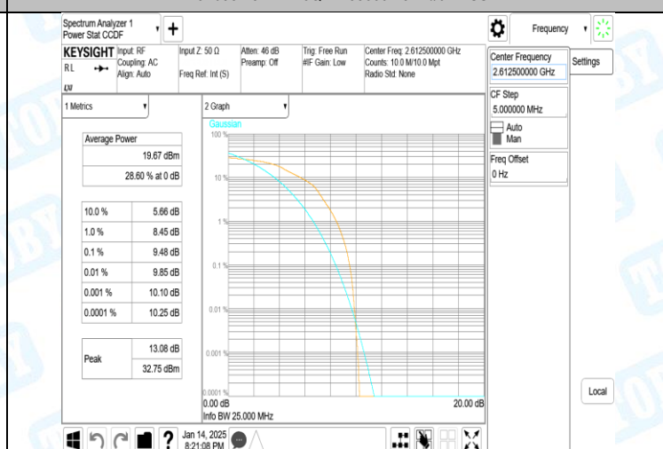
Band38-15MHz-16QAM-38175-75RB#0-PASS
