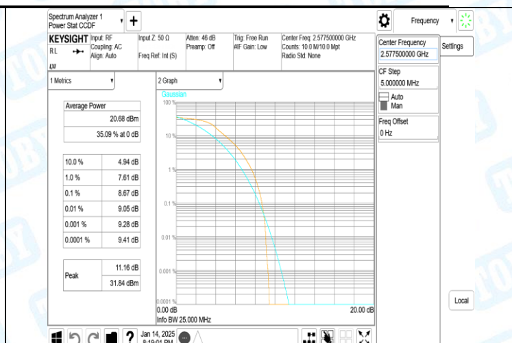
Band38-15MHz-QPSK-37825-75RB#0-PASS
