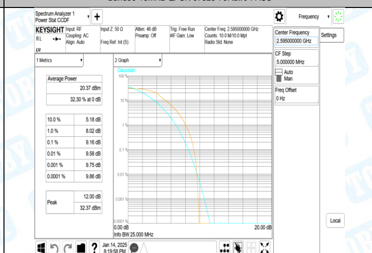
Band38-15MHz-QPSK-38000-75RB#0-PASS
