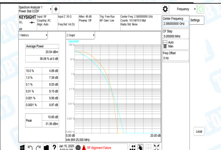
Band38-20MHz-QPSK-37850-100RB#0-PASS
