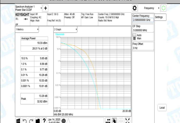
Band38-10MHz-16QAM-38000-50RB#0-PASS
