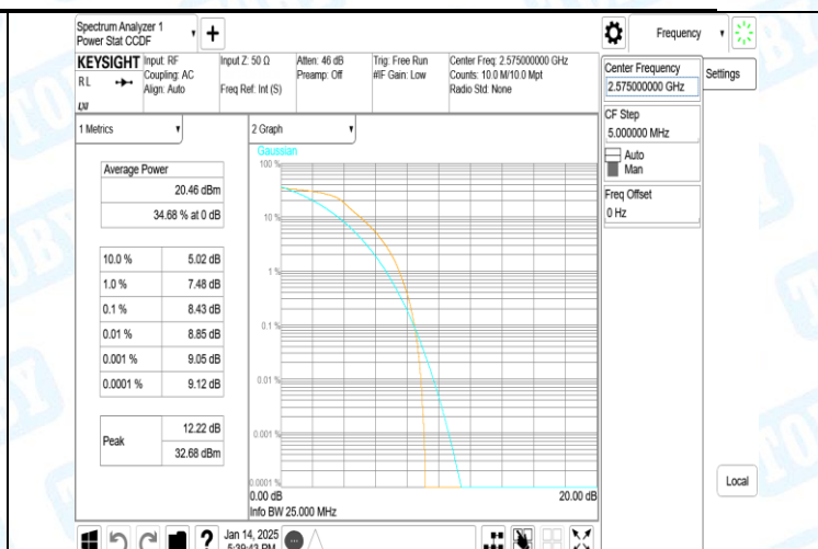
Band38-10MHz-QPSK-37800-50RB#0-PASS
