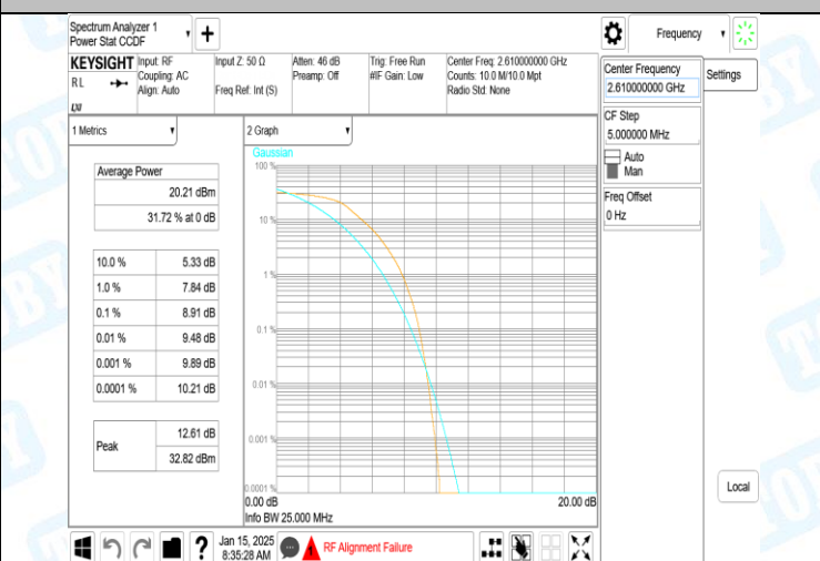
Band38-20MHz-QPSK-38150-100RB#0-PASS
