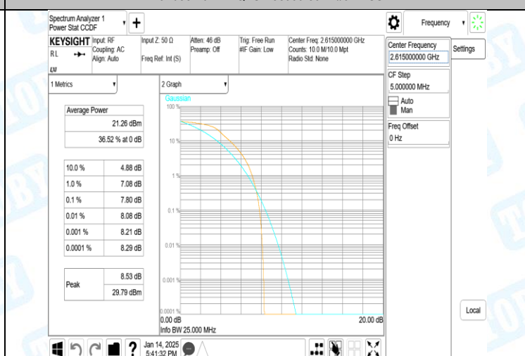
Band38-10MHz-QPSK-38200-50RB#0-PASS
