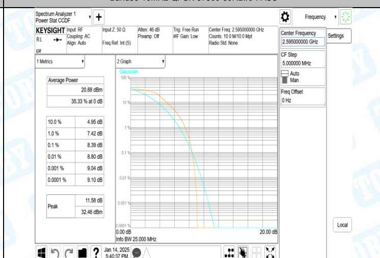
Band38-10MHz-QPSK-38000-50RB#0-PASS
