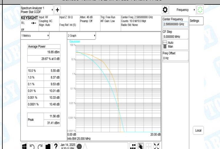
Band38-15MHz-16QAM-38000-75RB#0-PASS
