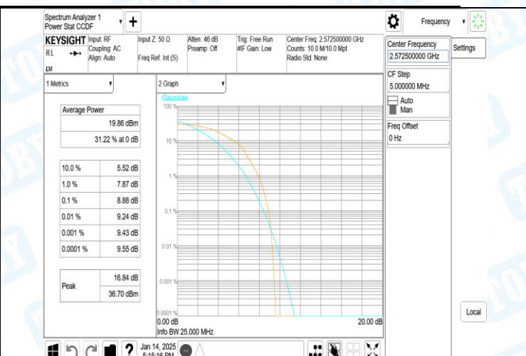
Band38-5MHz-16QAM-37775-25RB#0-PASS
