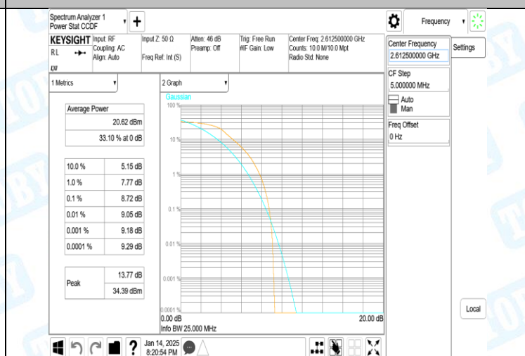
Band38-15MHz-QPSK-38175-75RB#0-PASS
