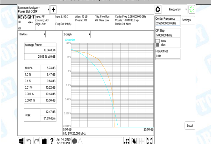
Band38-5MHz-16QAM-38000-25RB#0-PASS
