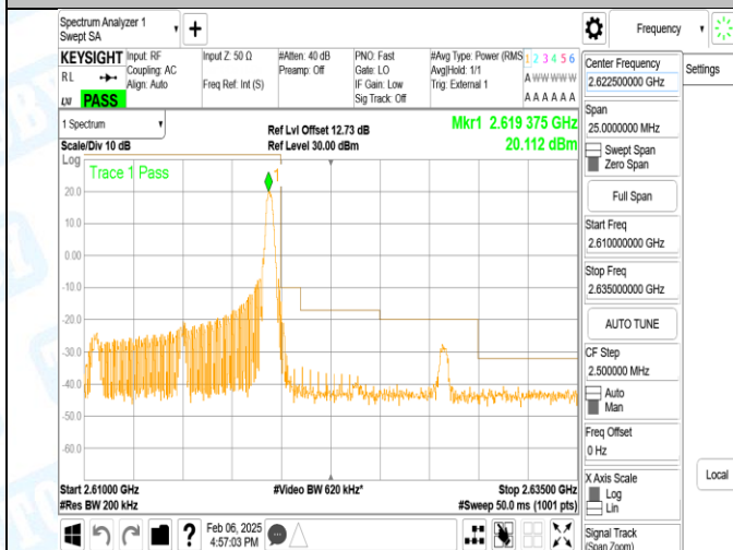
Band38_10MHz_QPSK_38200_1RB#49
