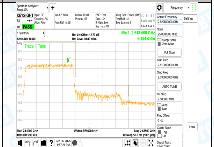
Band38_10MHz_QPSK_38200_50RB#0
