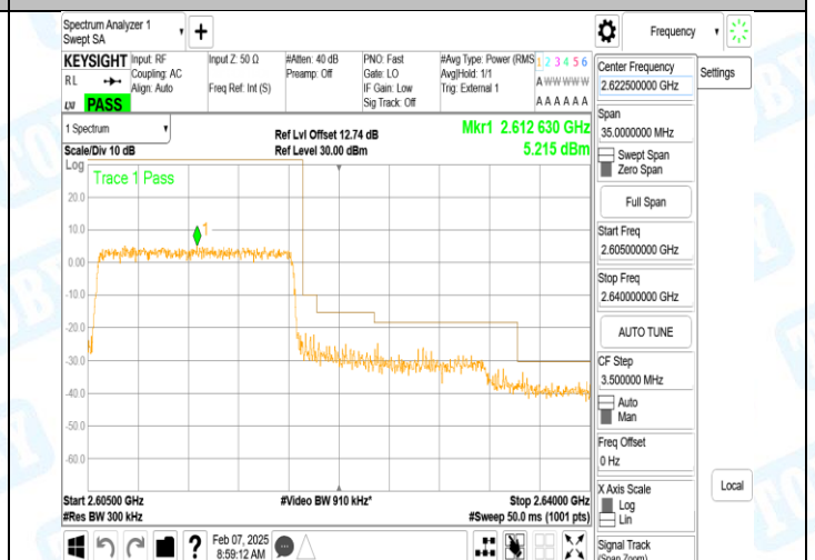
Band38_15MHz_QPSK_38175_1RB#0
