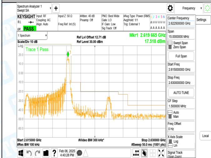
Band38_5MHz_16QAM_38225_1RB#24
