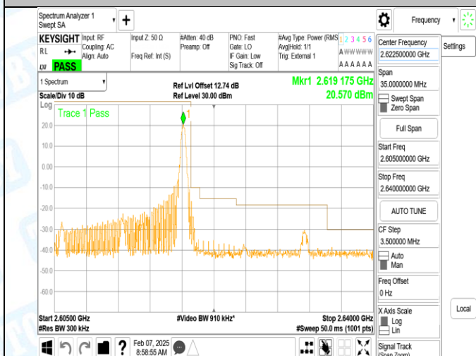
Band38_15MHz_QPSK_38175_1RB#74
