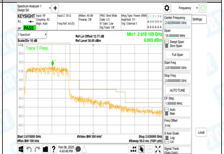
Band38_5MHz_16QAM_38225_25RB#0
