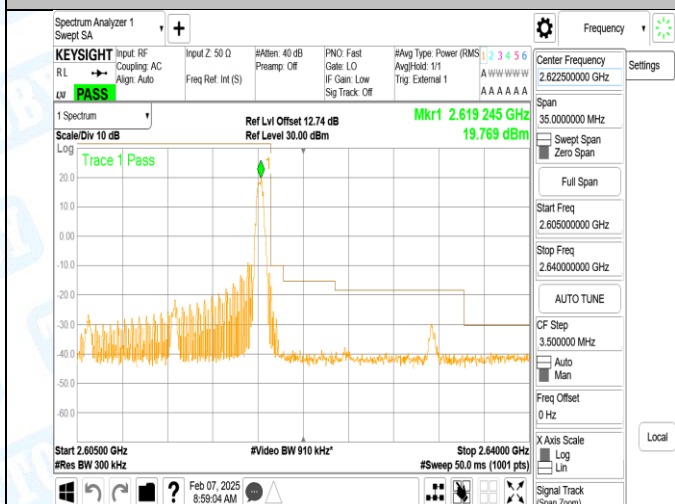
Band38_15MHz_16QAM_38175_1RB#74
