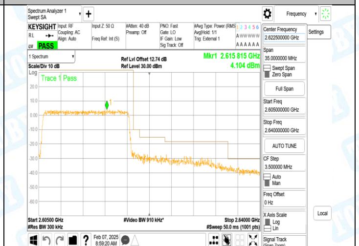
Band38_15MHz_16QAM_38175_75RB#0
