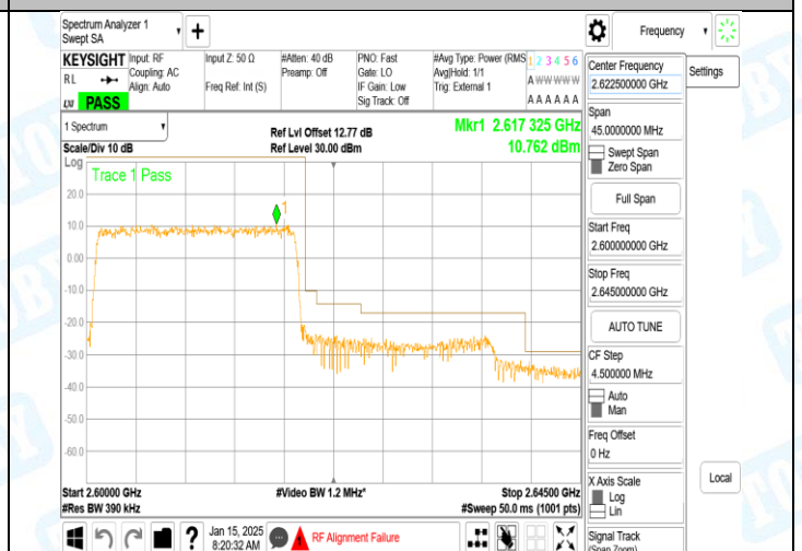
Band38_20MHz_QPSK_38150_100RB#0
