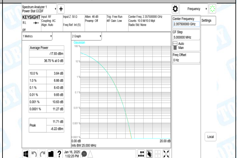
40(2350-2360)-5MHz-16QAM-39225-25RB#0-PASS
