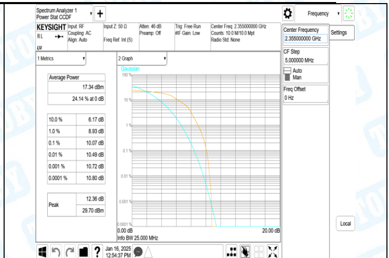
40(2350-2360)-5MHz-16QAM-39200-25RB#0-PASS
