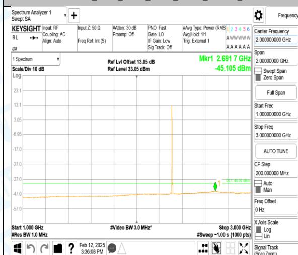
Band40_5MHz_QPSK_38750_1RB#0_1000~3000_1000~3000
