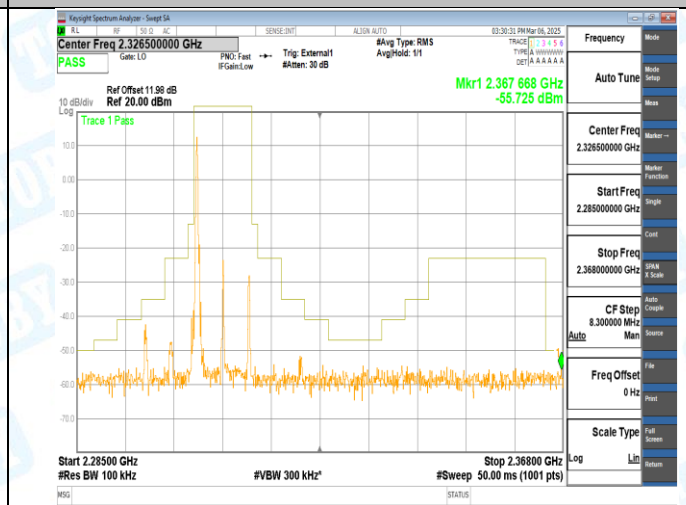
Band40_10MHz_QPSK_38750_50RB#49
