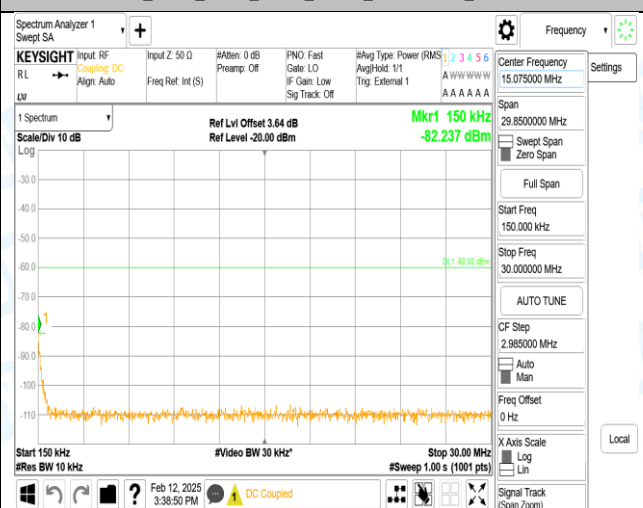
Band40_5MHz_QPSK_38775_1RB#0_0.15~30_0.15~30
