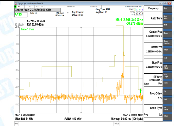
Band40_5MHz_QPSK_39175_1RB#24
