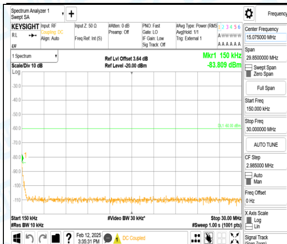
Band40_5MHz_QPSK_38750_1RB#0_0.15~30_0.15~30
