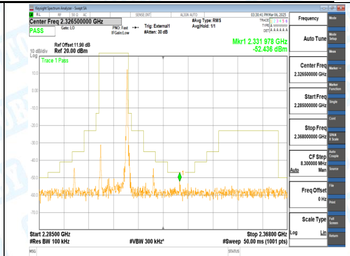
Band40_10MHz_QPSK_38750_1RB#49
