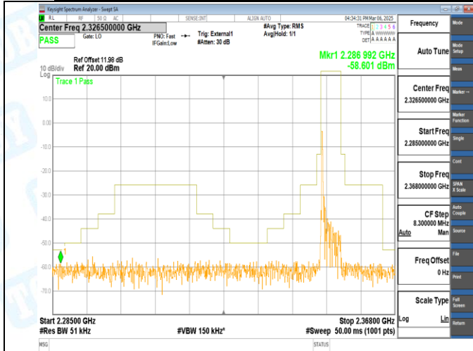
Band40_5MHz_QPSK_39175_1RB#0
