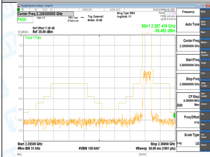
Band40_5MHz_QPSK_39175_25RB#0
