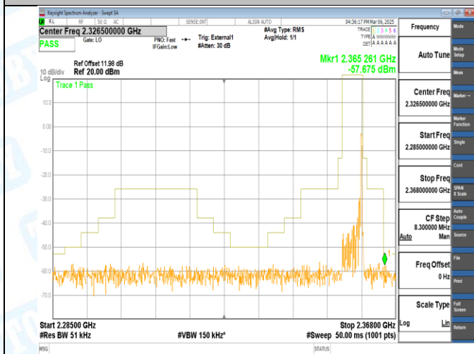
Band40_5MHz_QPSK_39225_1RB#24
