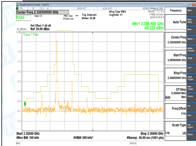
Band40_10MHz_QPSK_38750_1RB#0
