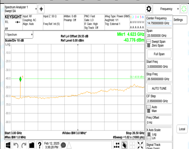
Band40_5MHz_QPSK_38750_1RB#0_3000~26500_3000~26500
