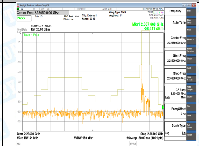
Band40_5MHz_QPSK_39225_1RB#0
