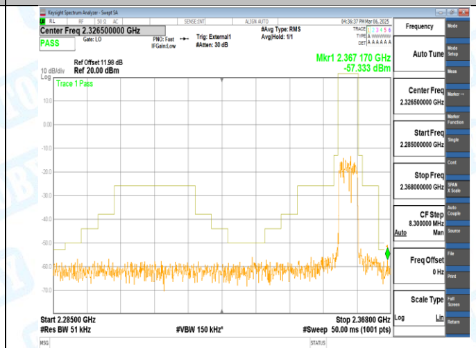
Band40_5MHz_QPSK_39225_25RB#0
