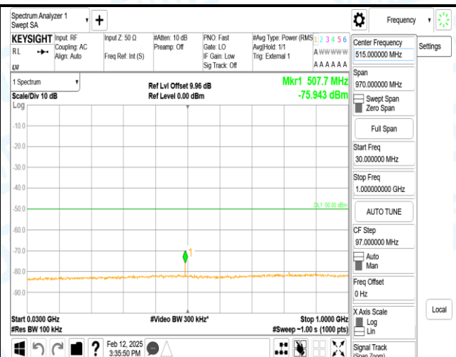
Band40_5MHz_QPSK_38750_1RB#0_30~1000_30~1000
