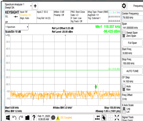
Band40_5MHz_16QAM_39200_1RB#0_0.009-0.15_0.009-0.15
