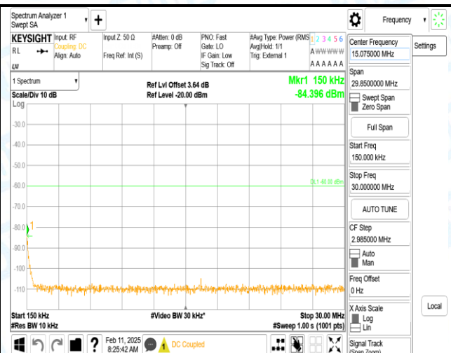
Band40_10MHz_QPSK_38750_1RB#0_0.15~30_0.15~30
