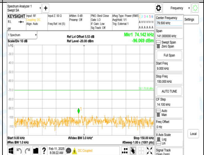
Band40_5MHz_16QAM_39225_1RB#0_0.009-0.15_0.009-0.15
