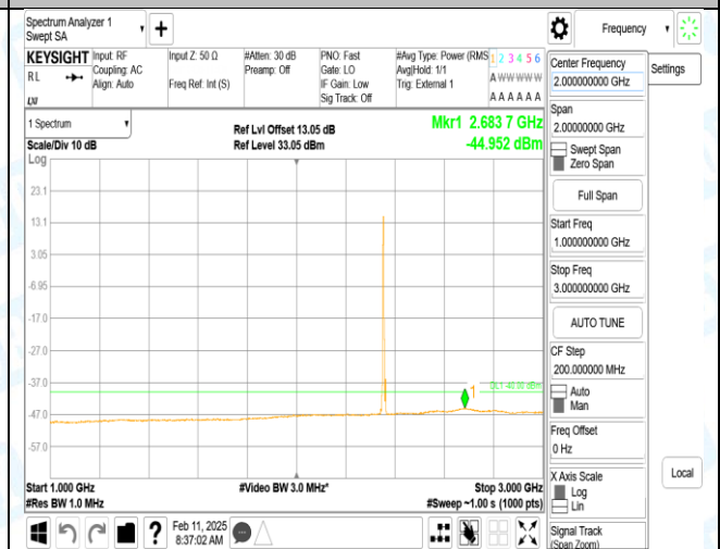
Band40_5MHz_16QAM_39200_1RB#0_1000-3000_1000-3000
