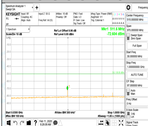
Band40_10MHz_QPSK_38750_1RB#0_30~1000_30~1000
