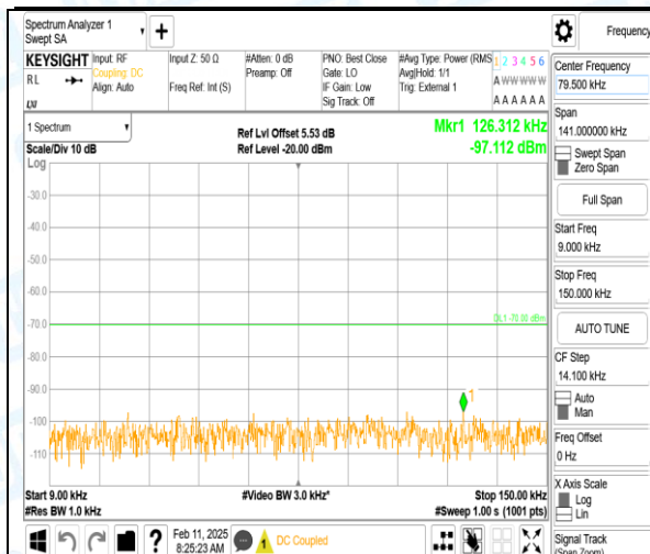
Band40_10MHz_QPSK_38750_1RB#0_0.009~0.15_0.009~0.15
