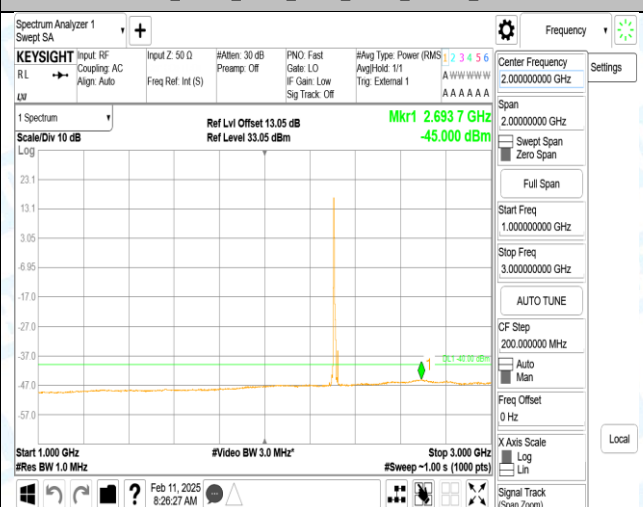
Band40_10MHz_QPSK_38750_1RB#0_1000~3000_1000~3000
