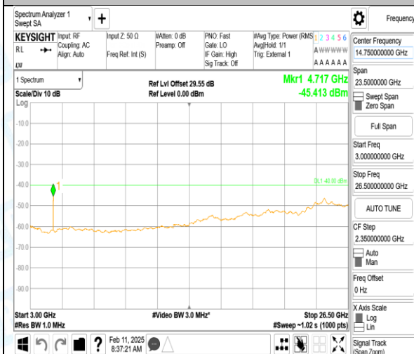
Band40_5MHz_16QAM_39200_1RB#0_3000-26500_3000-26500
