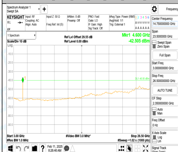
Band40_10MHz_QPSK_38750_1RB#0_3000~26500_3000~26500
