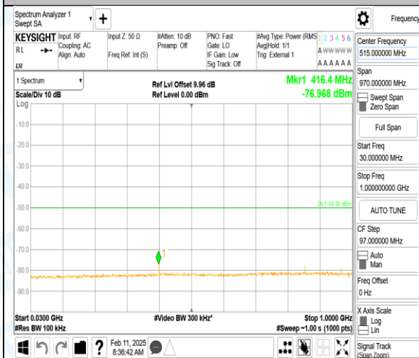
Band40_5MHz_16QAM_39200_1RB#0_30-1000_30-1000
