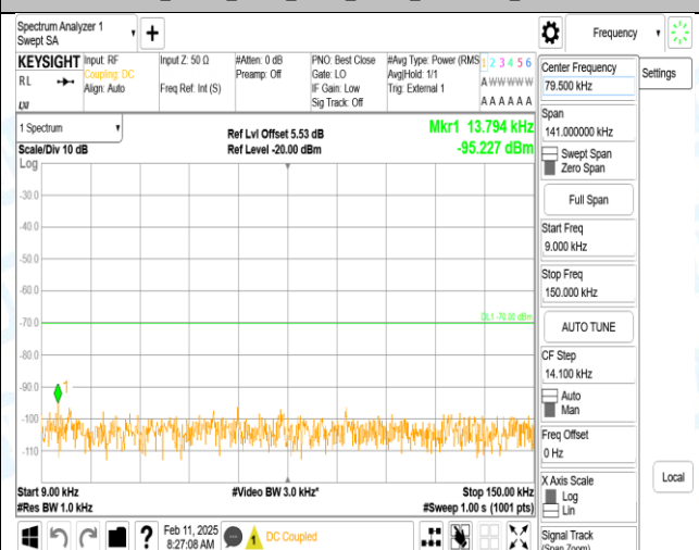
Band40_10MHz_16QAM_38750_1RB#0_0.009~0.15_0.009~0.15
