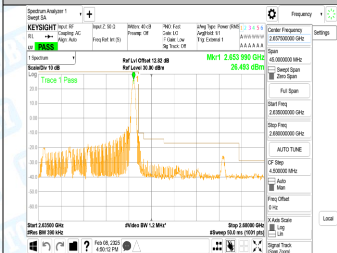
Band41_20MHz_QPSK_41140_1RB#99
