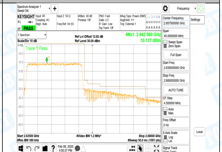
Band41_20MHz_16QAM_41140_100RB#0
