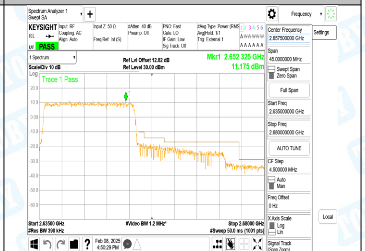
Band41_20MHz_QPSK_41140_100RB#0
