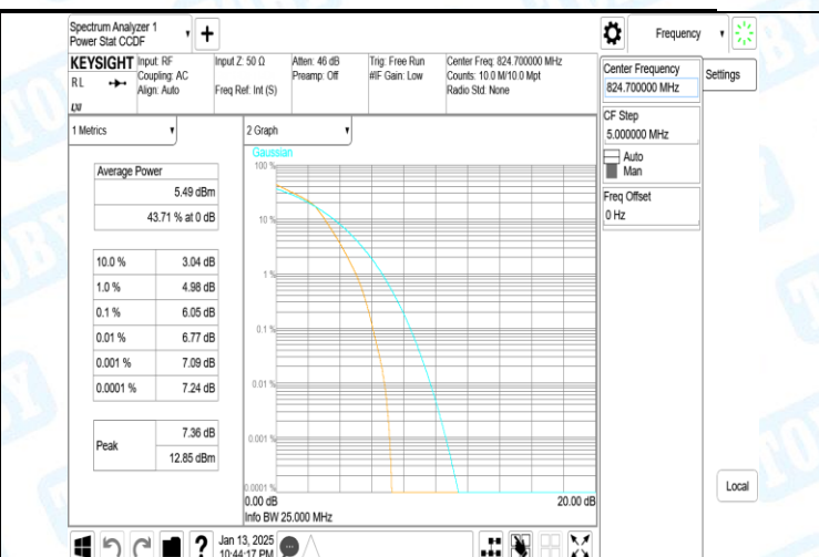
Band5-1.4MHz-16QAM-20407-6RB#0-PASS
