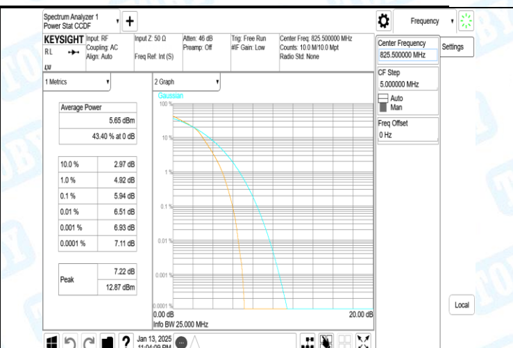
Band5-3MHz-16QAM-20415-15RB#0-PASS
