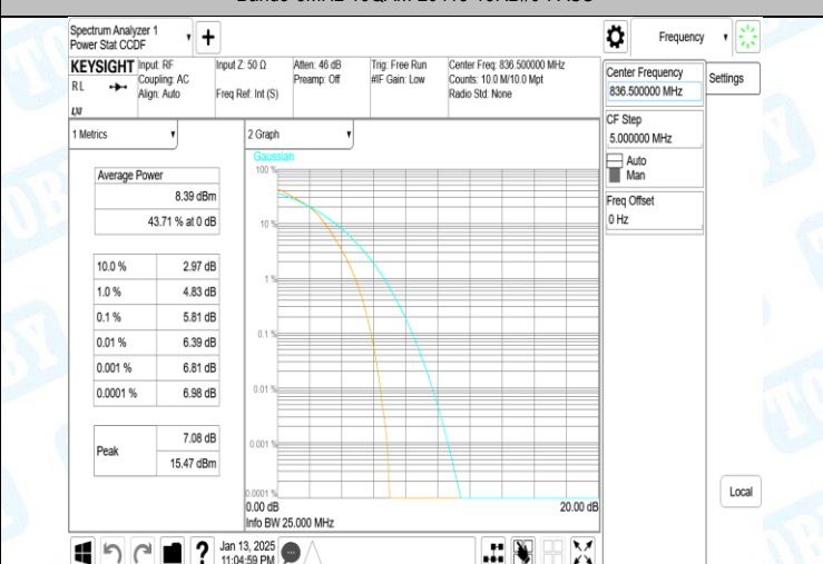
Band5-3MHz-16QAM-20525-15RB#0-PASS
