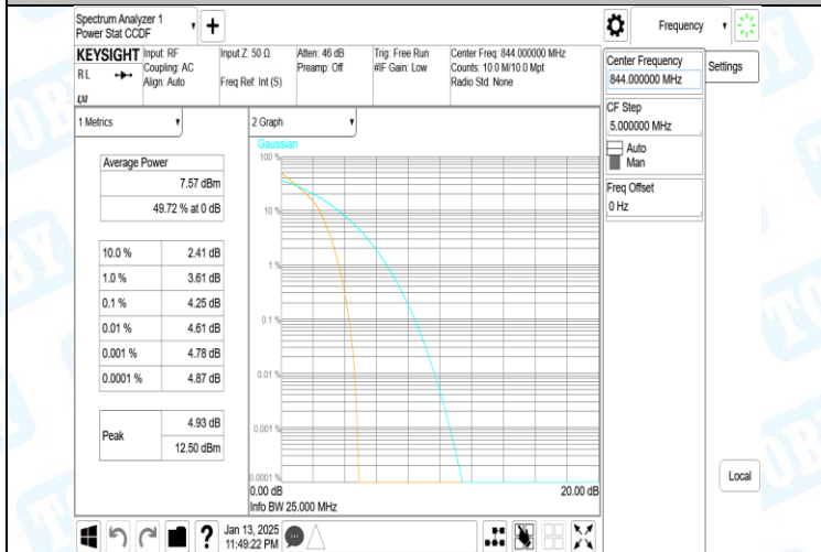
Band5-10MHz-QPSK-20600-1RB#0-PASS
