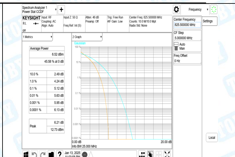
Band5-3MHz-QPSK-20415-15RB#0-PASS
