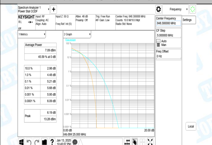
Band5-1.4MHz-16QAM-20643-6RB#0-PASS
