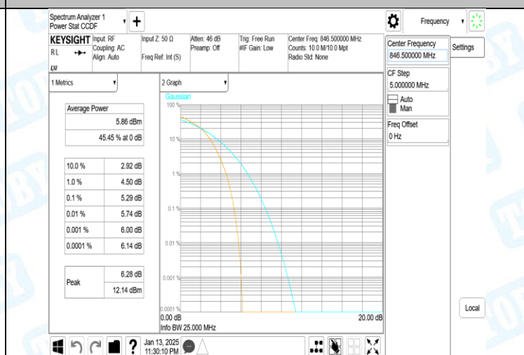
Band5-5MHz-16QAM-20625-25RB#0-PASS
