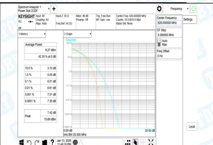
Band5-10MHz-16QAM-20450-50RB#0-PASS
