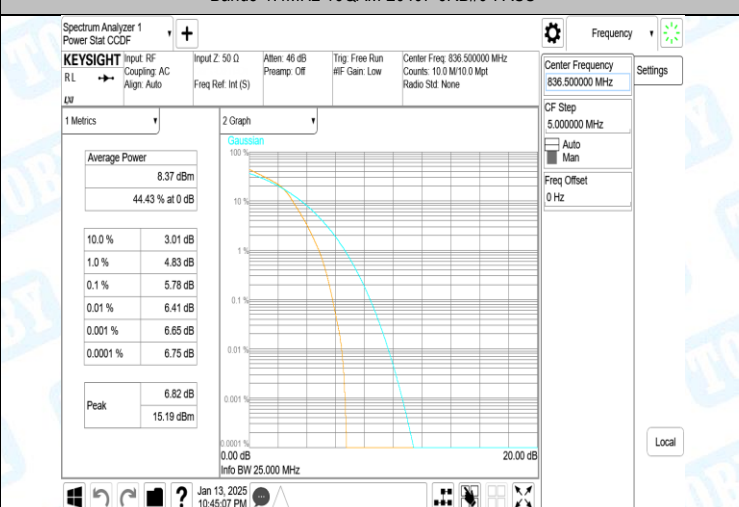
Band5-1.4MHz-16QAM-20525-6RB#0-PASS
