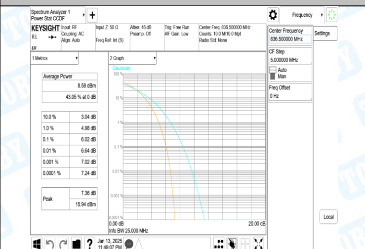
Band5-10MHz-16QAM-20525-50RB#0-PASS
