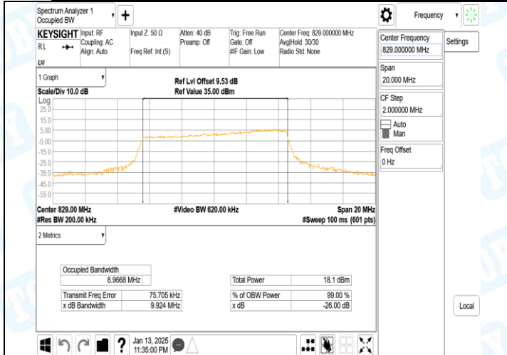
Band5-10MHz-QPSK-20450-50RB#0-PASS
