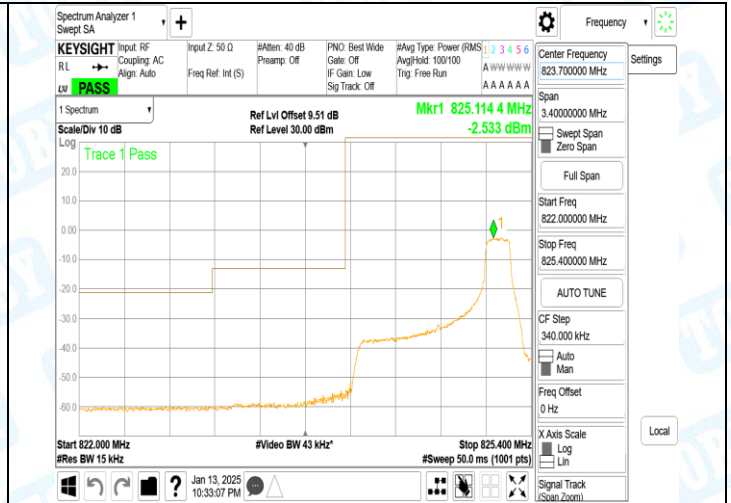
Band5_1.4MHz_QPSK_20407_1RB#5
