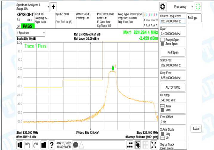
Band5_1.4MHz_QPSK_20407_1RB#0
