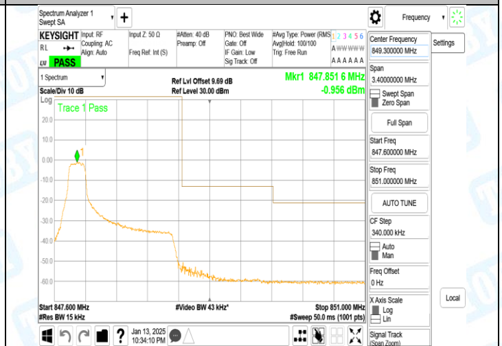
Band5_1.4MHz_QPSK_20643_1RB#0
