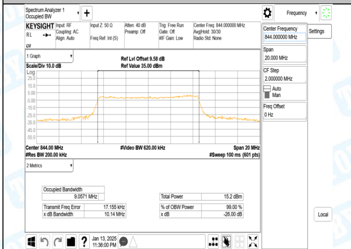
Band5-10MHz-QPSK-20600-50RB#0-PASS
