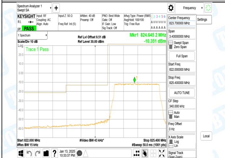
Band5_1.4MHz_QPSK_20407_6RB#0
