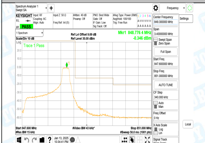
Band5_1.4MHz_QPSK_20643_1RB#5
