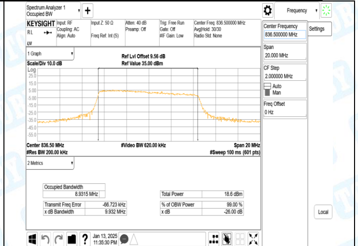
Band5-10MHz-QPSK-20525-50RB#0-PASS
