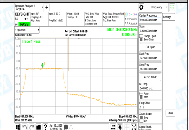
Band5_1.4MHz_QPSK_20643_6RB#0
