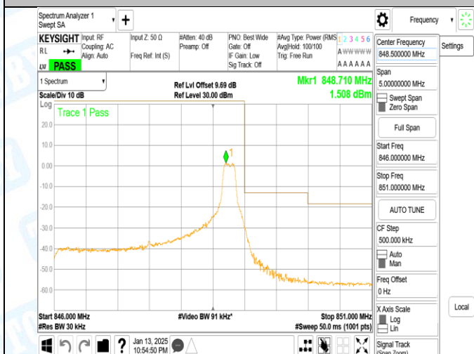
Band5_3MHz_16QAM_20635_15RB#14
