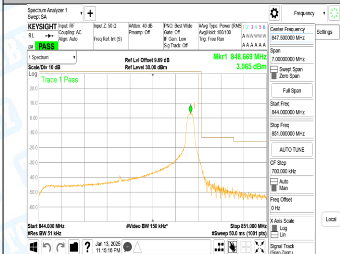
Band5_5MHz_16QAM_20625_1RB#24
