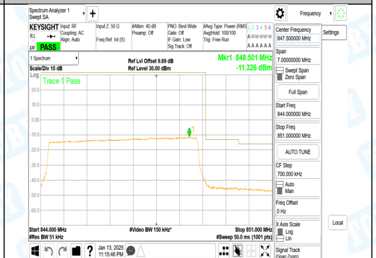
Band5_5MHz_16QAM_20625_25RB#0
