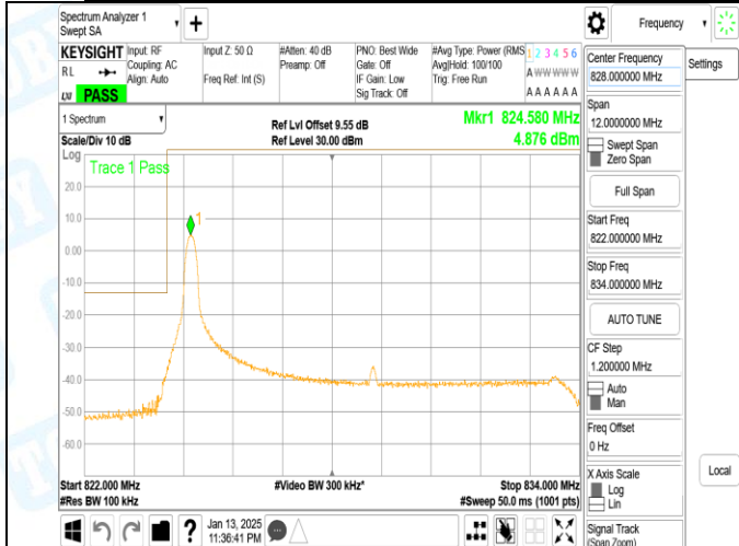
Band5_10MHz_QPSK_20450_1RB#0
