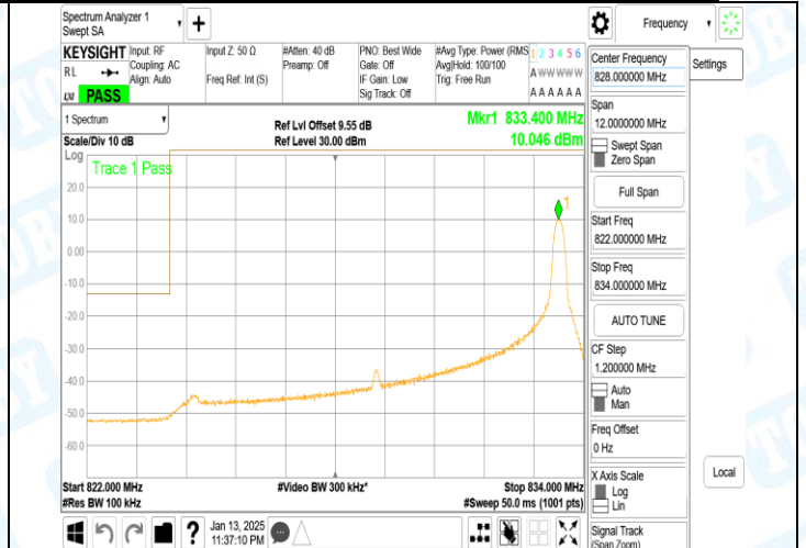
Band5_10MHz_QPSK_20450_1RB#49
