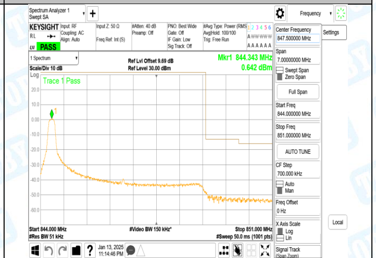
Band5_5MHz_16QAM_20625_1RB#0
