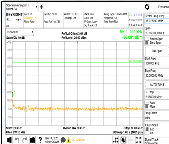
Band7_20MHz_QPSK_21100_1RB#0_0.15~30_0.15~30
