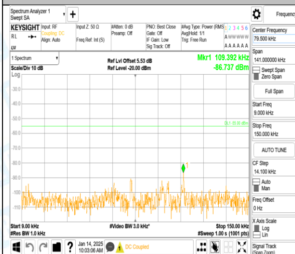
Band7_20MHz_QPSK_21350_1RB#0_0.009~0.15_0.009~0.15
