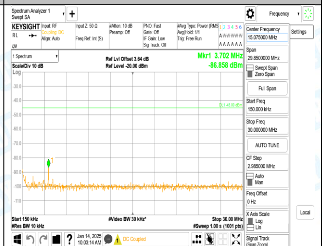
Band7_20MHz_QPSK_21350_1RB#0_0.15~30_0.15~30
