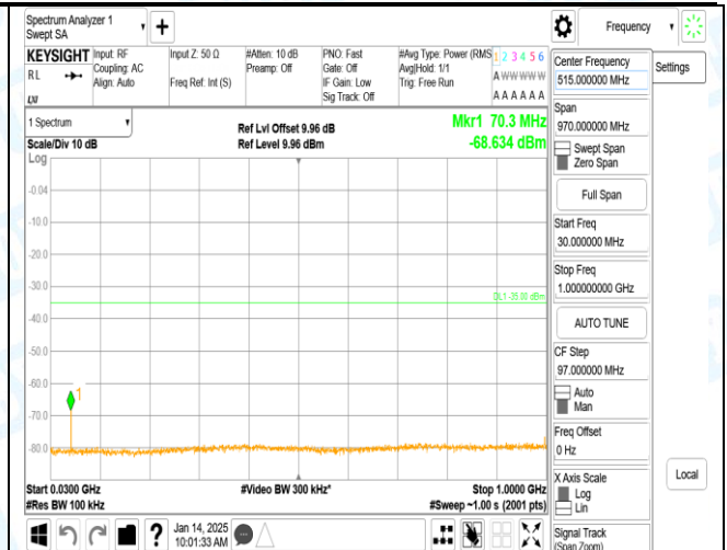
Band7_20MHz_QPSK_21100_1RB#0_30~1000_30~1000
