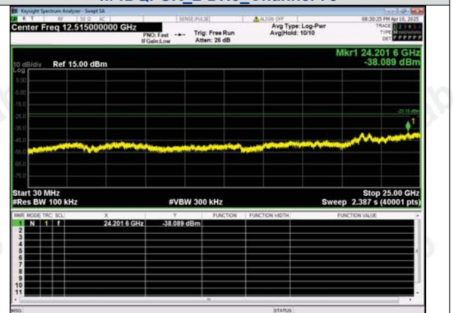
30.0 MHz - 25000.0 MHz \pi/4 DQPSK_2-DH5_Channel 78
