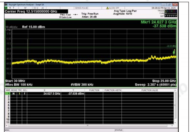
30.0 MHz - 25000.0 MHz \pi/4 DQPSK_2-DH5_Channel 39
