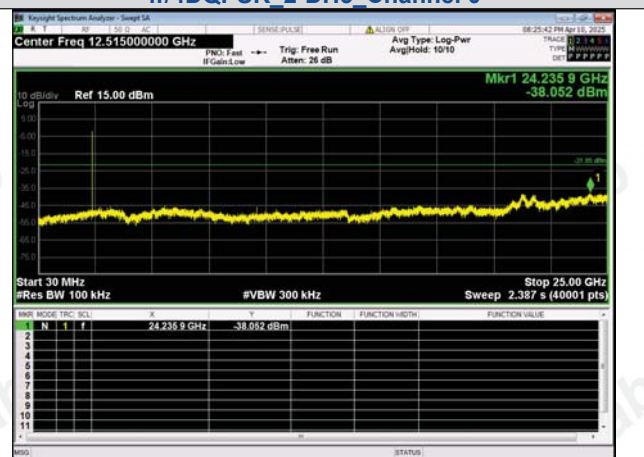
30.0 MHz - 25000.0 MHz \pi/4 DQPSK_2-DH5_Channel 0
