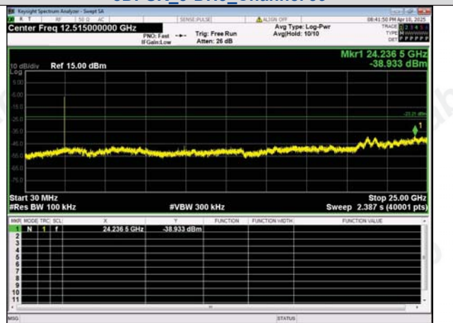
30.0 MHz - 25000.0 MHz 8DPSK_3-DH5_Channel 78
