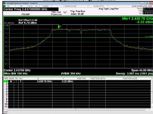
Band edge Emission,11g(HT20),Middle
