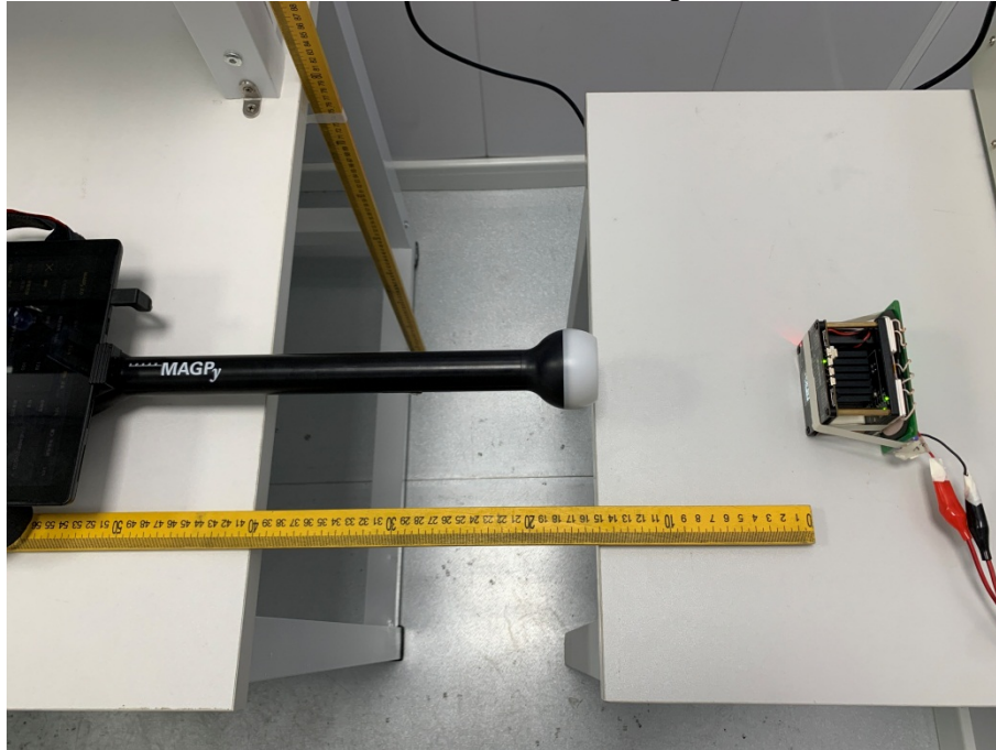
EUT distance from load 5 mm H-Field and E-Field Strength
