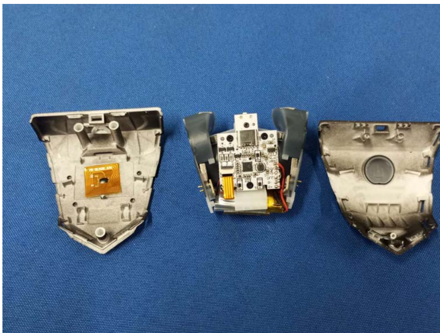
Photo 1- charger base
