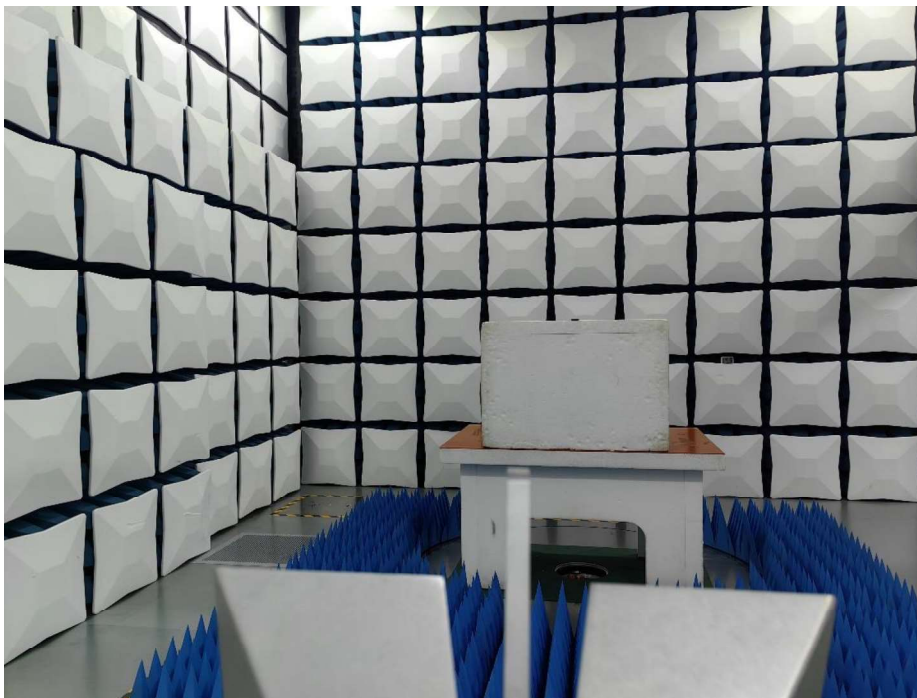
Test Set-up: Radiated spurious emission 1GHz-18GHz
