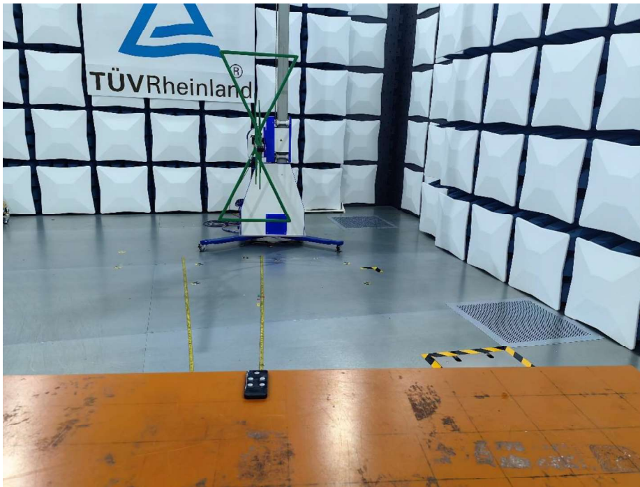
Test Set-up: Radiated spurious emission Below 1GHz
