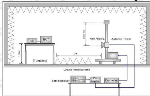
Figure 3. Above 1GHz
