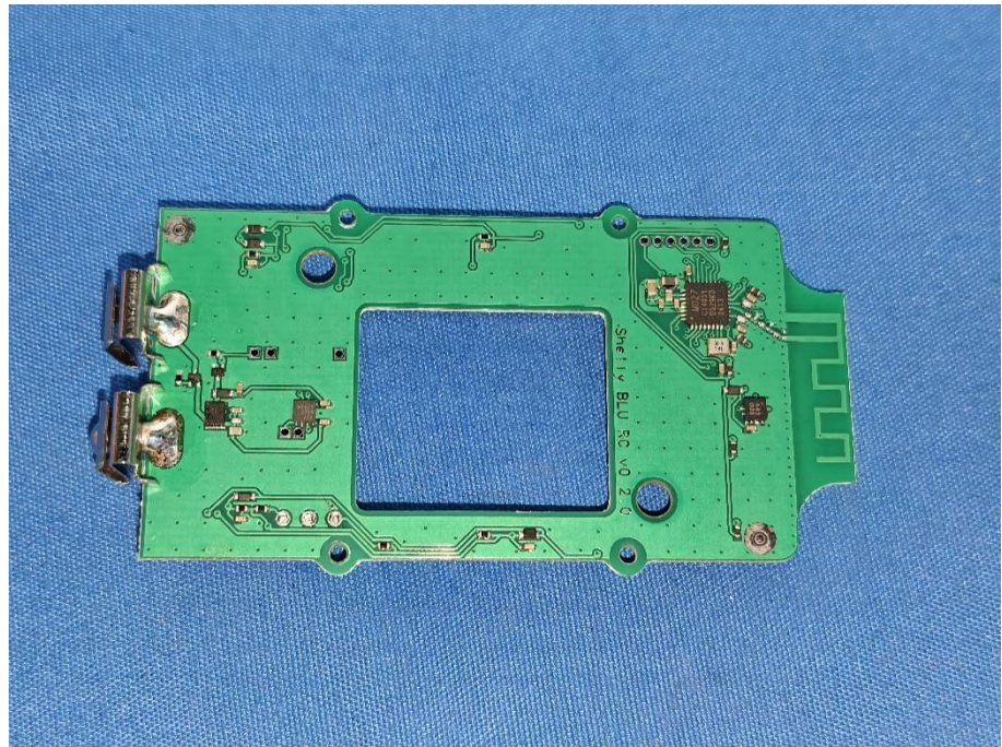
Bluetooth/Zigbee Antenna
