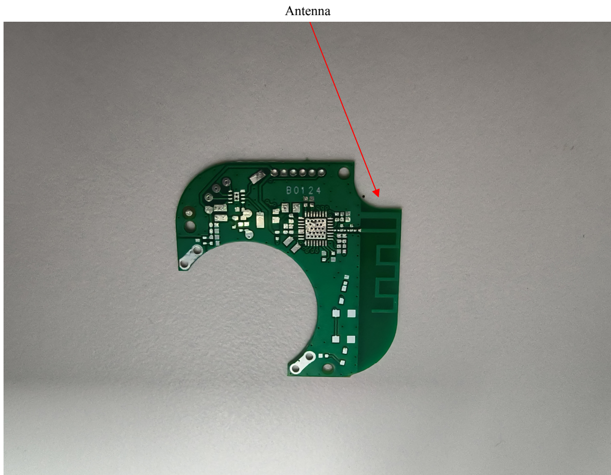
Antenna dimension
