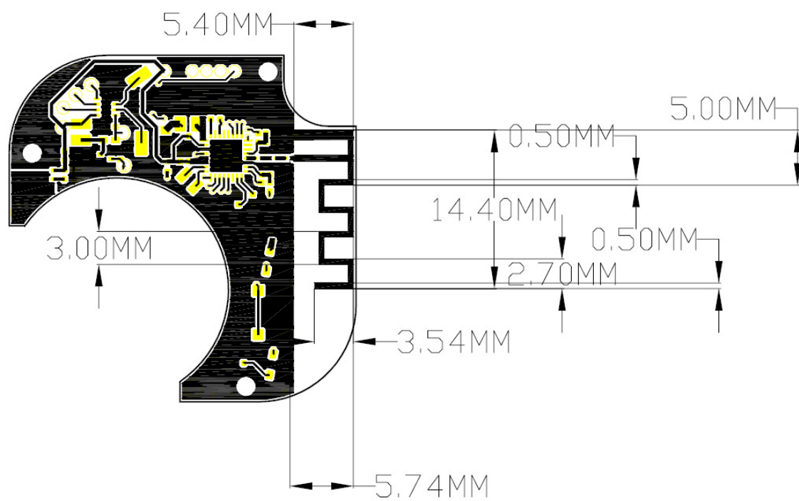
Antenna dimension
